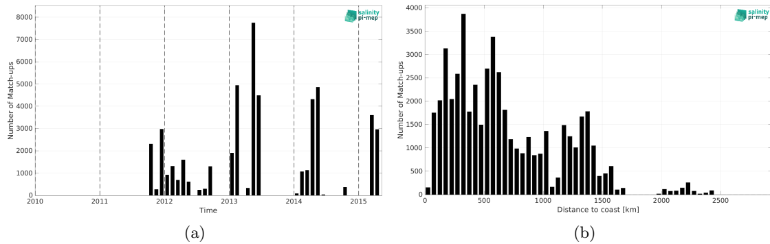
Figure 2: Number of match-ups between TSG (GOSUD-Research-vessel) and Aquarius SSS L2 OR v5 (NASA-GSFC) SSS as a function of time (a) and as function of the distance to coast (b) over the Equatorial Ocean 10N-10S Pi-MEP region and for the full satellite product period.
