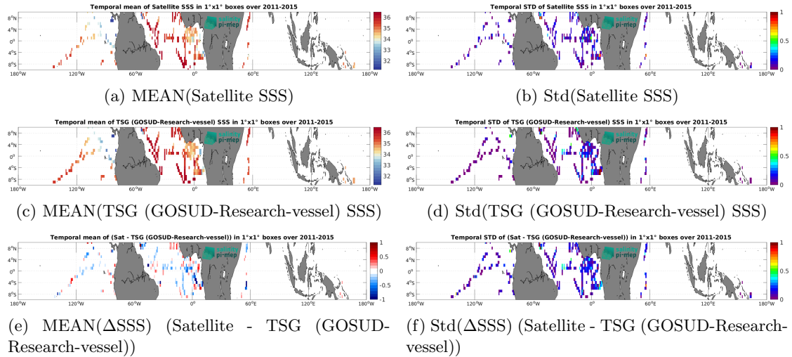
Figure 7: Temporal mean (left) and Std (right) of SSS from Aquarius SSS L2 OR v5 (NASA-GSFC) (top), TSG (GOSUD-Research-vessel) (middle), and of \Delta SSS (Satellite - TSG (GOSUD-Research-vessel)). Only match-up pairs are used to generate these maps.
