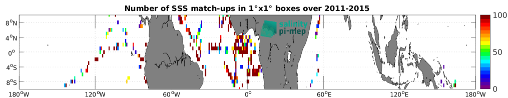
Figure 5: Number of SSS match-ups between TSG (GOSUD-Research-vessel) SSS and the Aquarius SSS L2 OR v5 (NASA-GSFC) SSS product for the Equatorial Ocean 10N-10S Pi-MEP region over 1^\circ \times 1^\circ boxes and for the full satellite product period.
