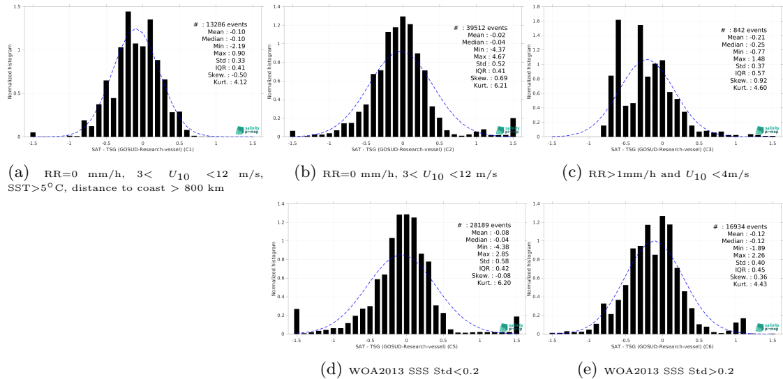
Figure 15: Normalized histogram of \Delta\text{SSS} (Aquarius SSS L2 OR v5 (NASA-GSFC) - TSG (GOSUD-Research-vessel)) for 5 different subdatasets corresponding to: RR=0 mm/h, 3 < U_{10} < 12 m/s, SST>5°C, distance to coast > 800 km (a), RR=0 mm/h, 3 < U_{10} < 12 m/s (b), RR>1mm/h and U_{10} < 4 m/s (c), WOA2013 SSS Std<0.2 (d), WOA2013 SSS Std>0.2 (e).
