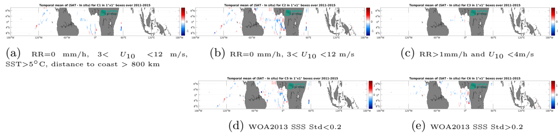
Figure 14: Temporal mean gridded over spatial boxes of size 1^\circ \times 1^\circ of \Delta\text{SSS} (Aquarius SSS L2 OR v5 (NASA-GSFC) - TSG (GOSUD-Research-vessel)) for 5 different subdatasets corresponding to: RR=0 mm/h, 3 < U_{10} < 12 m/s, SST>5°C, distance to coast > 800 km (a), RR=0 mm/h, 3 < U_{10} < 12 m/s (b), RR>1mm/h and U_{10} < 4 m/s (c), WOA2013 SSS Std<0.2 (d), WOA2013 SSS Std>0.2 (e).
