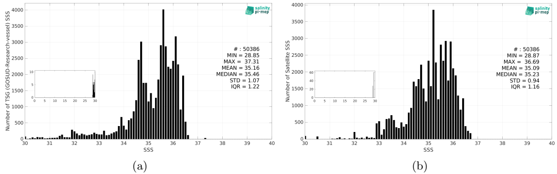
Figure 3: Histograms of SSS from TSG (GOSUD-Research-vessel) (a) and Aquarius SSS L2 OR v5 (NASA-GSFC) (b) considering all match-up pairs per bins of 0.1 over the Equatorial Ocean 10N-10S Pi-MEP region and for the full satellite product period.
