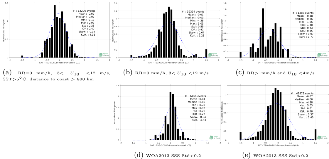
Figure 13: Normalized histogram of \Delta SSS (Aquarius-L2-OR-V5 - TSG-GOSUD-Research-vessel) for 5 different subdatasets corresponding to: RR=0 mm/h, 3 < U_{10} < 12 m/s, SST >5^\circ\text{C} , distance to coast > 800 km (a), RR=0 mm/h, 3 < U_{10} < 12 m/s (b), RR >1 mm/h and U_{10} < 4 m/s (c), WOA2013 SSS Std <0.2 (d), WOA2013 SSS Std >0.2 (e).
