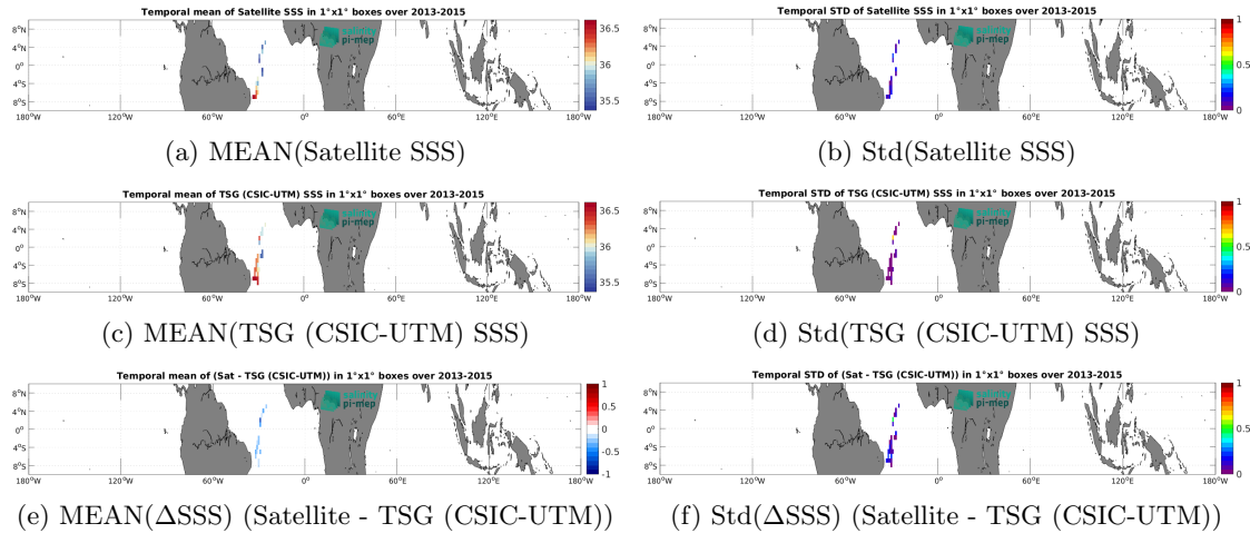
Figure 7: Temporal mean (left) and Std (right) of SSS from Aquarius SSS L2 OR v5 (NASA-GSFC) (top), TSG (CSIC-UTM) (middle), and of \Delta SSS (Satellite - TSG (CSIC-UTM)). Only match-up pairs are used to generate these maps.
