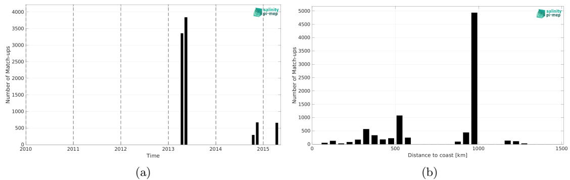
Figure 2: Number of match-ups between TSG (CSIC-UTM) and Aquarius SSS L2 OR v5 (NASA-GSFC) SSS as a function of time (a) and as function of the distance to coast (b) over the Equatorial Ocean 10N-10S Pi-MEP region and for the full satellite product period.
