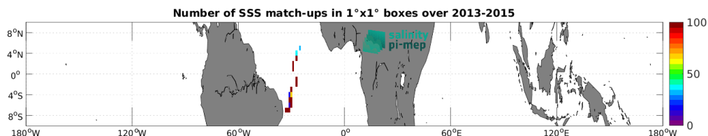
Figure 5: Number of SSS match-ups between TSG (CSIC-UTM) SSS and the Aquarius SSS L2 OR v5 (NASA-GSFC) SSS product for the Equatorial Ocean 10N-10S Pi-MEP region over 1^\circ \times 1^\circ boxes and for the full satellite product period.
