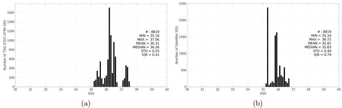
Figure 3: Histograms of SSS from TSG (CSIC-UTM) (a) and Aquarius SSS L2 OR v5 (NASA-GSFC) (b) considering all match-up pairs per bins of 0.1 over the Equatorial Ocean 10N-10S Pi-MEP region and for the full satellite product period.
