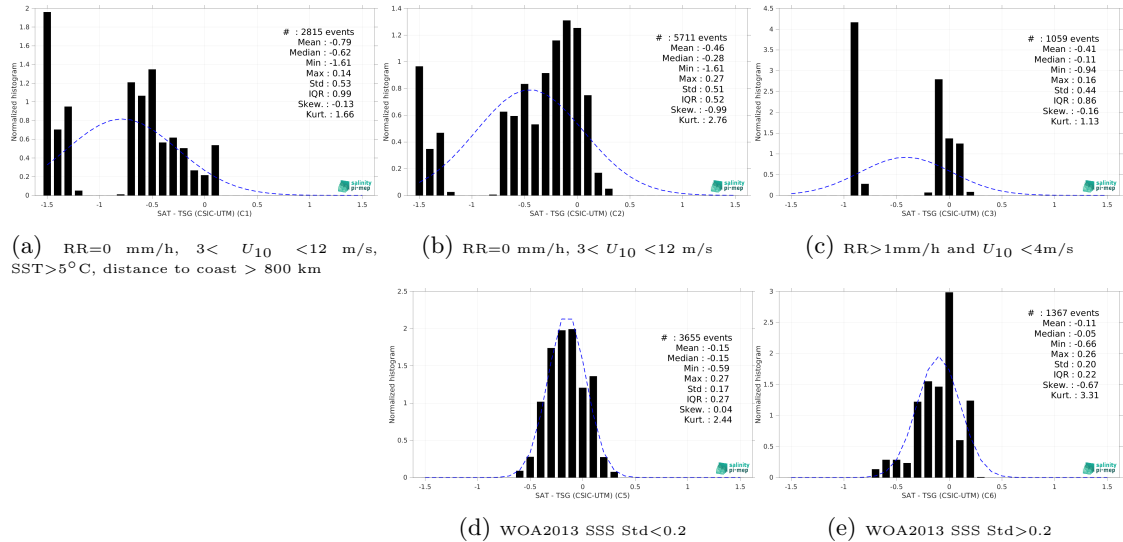
Figure 13: Normalized histogram of \Delta SSS (Aquarius SSS L2 OR v5 (NASA-GSFC) - TSG (CSIC-UTM)) for 5 different subdatasets corresponding to: RR=0 mm/h, 3 < U_{10} < 12 m/s, SST >5^\circ\text{C} , distance to coast > 800 km (a), RR=0 mm/h, 3 < U_{10} < 12 m/s (b), RR >1 mm/h and U_{10} < 4 m/s (c), WOA2013 SSS Std <0.2 (d), WOA2013 SSS Std >0.2 (e).
