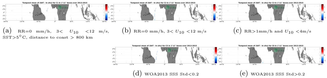
Figure 12: Temporal mean gridded over spatial boxes of size 1^\circ \times 1^\circ of \Delta SSS (Aquarius SSS L2 OR v5 (NASA-GSFC) - TSG (CSIC-UTM)) for 5 different subdatasets corresponding to: RR=0 mm/h, 3 < U_{10} < 12 m/s, SST>5°C, distance to coast > 800 km (a), RR=0 mm/h, 3 < U_{10} < 12 m/s (b), RR>1mm/h and U_{10} < 4 m/s (c), WOA2013 SSS Std<0.2 (d), WOA2013 SSS Std>0.2 (e).
