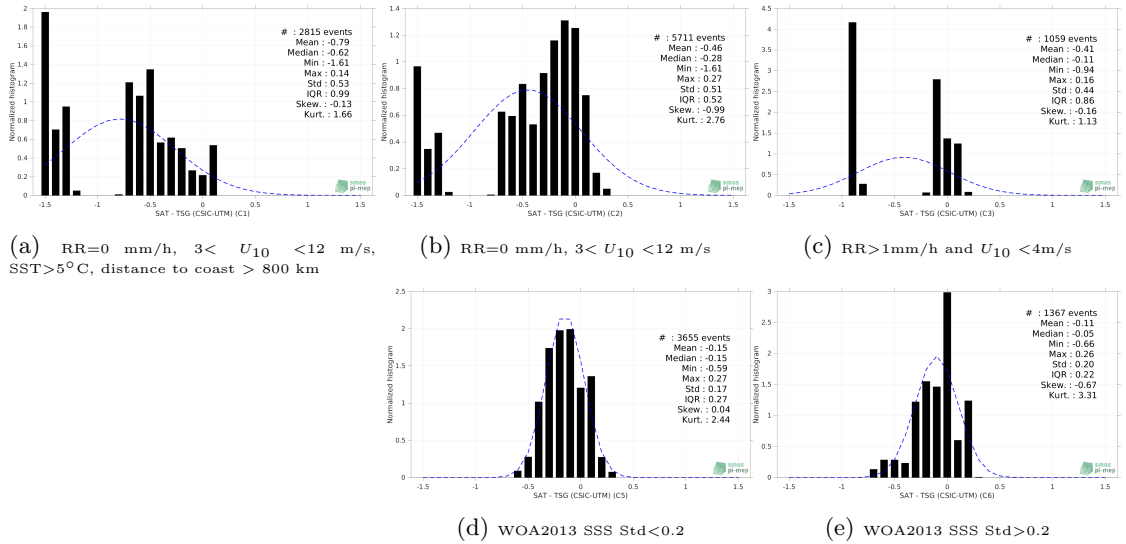
Figure 13: Normalized histogram of \Delta SSS (Aquarius SSS L2 OR v5 (NASA-GSFC) - TSG (CSIC-UTM)) for 5 different subdatasets corresponding to: RR=0 mm/h, 3 < U_{10} < 12 m/s, SST>5°C, distance to coast > 800 km (a), RR=0 mm/h, 3 < U_{10} < 12 m/s (b), RR>1mm/h and U_{10} < 4 m/s (c), WOA2013 SSS Std<0.2 (d), WOA2013 SSS Std>0.2 (e).
