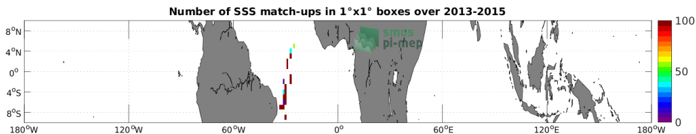
Figure 4: Number of SSS match-ups between TSG (CSIC-UTM) SSS and the Aquarius SSS L2 OR v5 (NASA-GSFC) SSS product for the Equatorial Ocean 10N-10S Pi-MEP region over 1^\circ \times 1^\circ boxes and for the full satellite product period.
