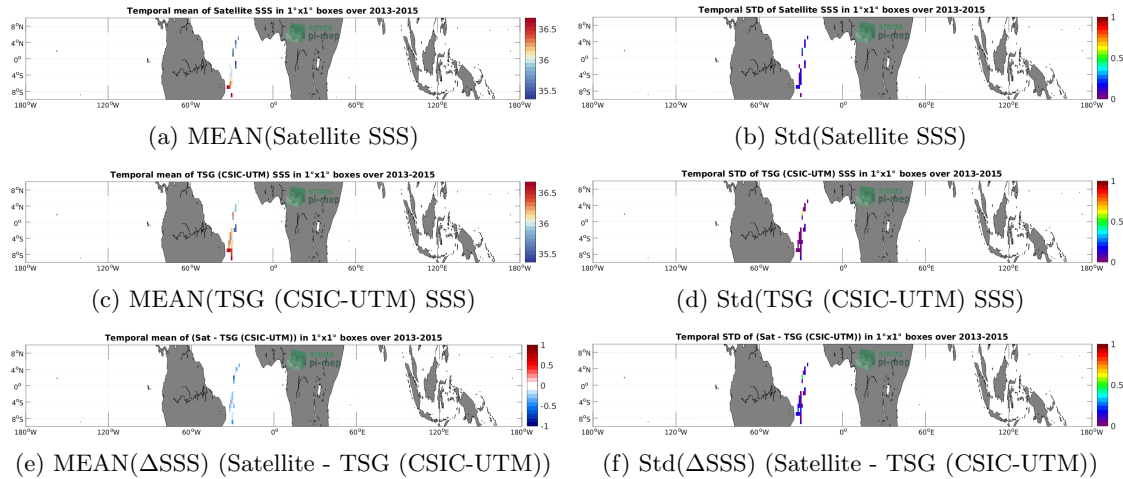
Figure 6: Temporal mean (left) and Std (right) of SSS from Aquarius SSS L2 OR v5 (NASA-GSFC) (top), TSG (CSIC-UTM) (middle), and of \Delta SSS (Satellite - TSG (CSIC-UTM)). Only match-up pairs are used to generate these maps.
