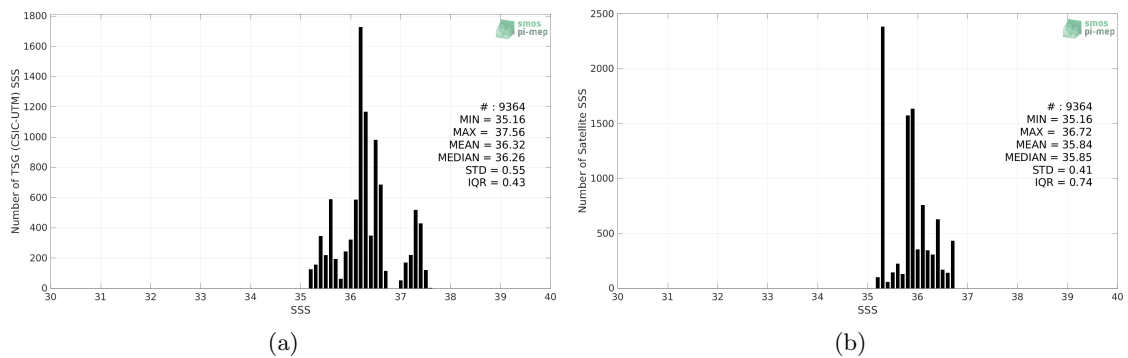
Figure 2: Histograms of SSS from TSG (CSIC-UTM) (a) and Aquarius SSS L2 OR v5 (NASA-GSFC) (b) considering all match-up pairs per bins of 0.1 over the Equatorial Ocean 10N-10S Pi-MEP region and for the full satellite product period.
