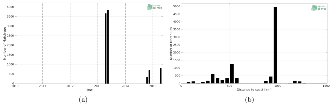
Figure 1: Number of match-ups between TSG (CSIC-UTM) and Aquarius SSS L2 OR v5 (NASA-GSFC) SSS as a function of time (a) and as function of the distance to coast (b) over the Equatorial Ocean 10N-10S Pi-MEP region and for the full satellite product period.
