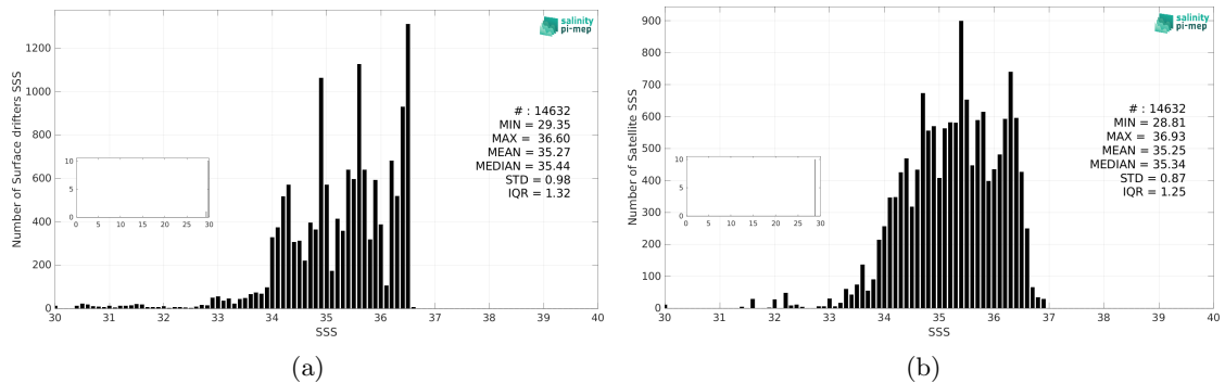
Figure 3: Histograms of SSS from Surface drifters (a) and Aquarius SSS L2 OR v5 (NASA-GSFC) (b) considering all match-up pairs per bins of 0.1 over the Equatorial Ocean 10N-10S Pi-MEP region and for the full satellite product period.
