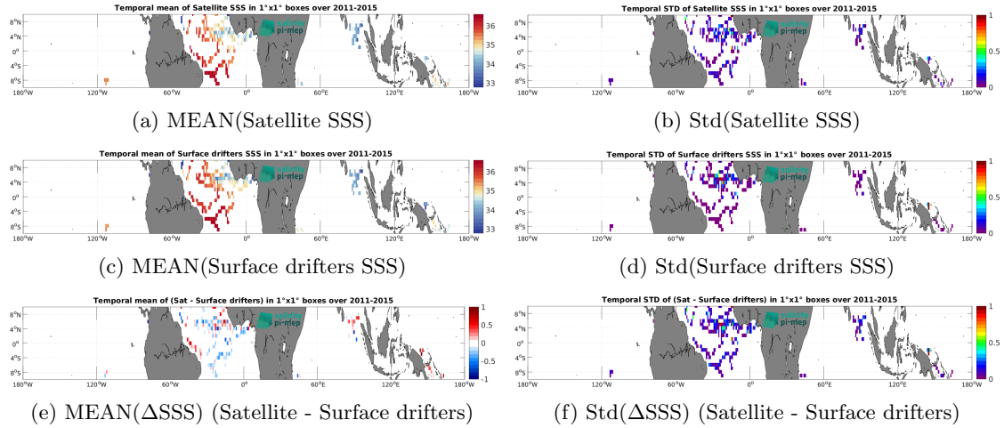
Figure 6: Temporal mean (left) and Std (right) of SSS from Aquarius SSS L2 OR v5 (NASA-GSFC) (top), Surface drifters (middle), and of \Delta SSS (Satellite - Surface drifters). Only match-up pairs are used to generate these maps.
