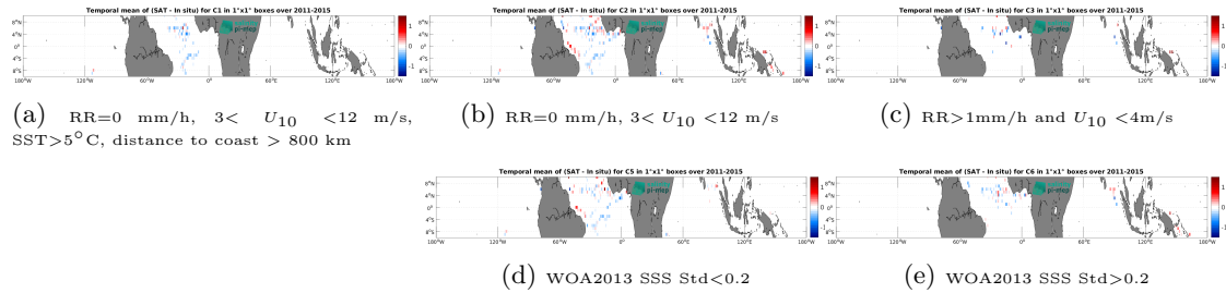
Figure 13: Temporal mean gridded over spatial boxes of size 1^\circ \times 1^\circ of \Delta SSS (Aquarius SSS L2 OR v5 (NASA-GSFC) - Surface drifters) for 5 different subdatasets corresponding to: RR=0 mm/h, 3 < U_{10} < 12 m/s, SST >5^\circ C, distance to coast > 800 km (a), RR=0 mm/h, 3 < U_{10} < 12 m/s (b), RR >1 mm/h and U_{10} < 4 m/s (c), WOA2013 SSS Std <0.2 (d), WOA2013 SSS Std >0.2 (e).
