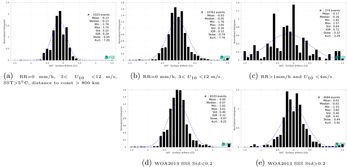
Figure 14: Normalized histogram of \Delta SSS (Aquarius SSS L2 OR v5 (NASA-GSFC) - Surface drifters) for 5 different subdatasets corresponding to: RR=0 mm/h, 3 < U_{10} < 12 m/s, SST >5^\circ C, distance to coast > 800 km (a), RR=0 mm/h, 3 < U_{10} < 12 m/s (b), RR >1 mm/h and U_{10} < 4 m/s (c), WOA2013 SSS Std <0.2 (d), WOA2013 SSS Std >0.2 (e).
