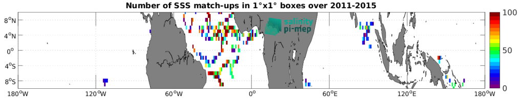
Figure 4: Number of SSS match-ups between Surface drifters SSS and the Aquarius SSS L2 OR v5 (NASA-GSFC) SSS product for the Equatorial Ocean 10N-10S Pi-MEP region over 1^\circ \times 1^\circ boxes and for the full satellite product period.
