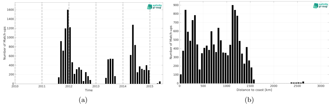
Figure 2: Number of match-ups between Surface drifters and Aquarius SSS L2 OR v5 (NASA-GSFC) SSS as a function of time (a) and as function of the distance to coast (b) over the Equatorial Ocean 10N-10S Pi-MEP region and for the full satellite product period.
