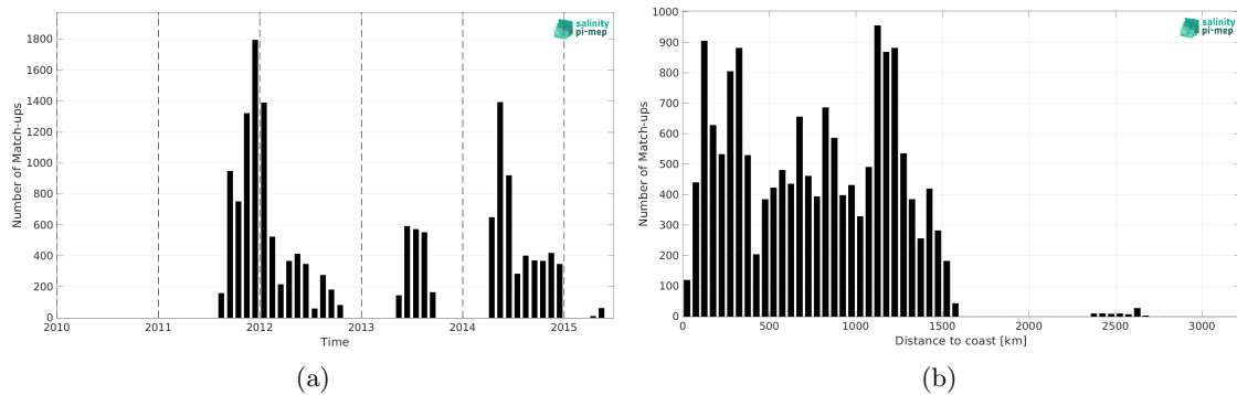
Figure 1: Number of match-ups between Surface drifters and Aquarius SSS L2 OR v5 (NASA-GSFC) SSS as a function of time (a) and as function of the distance to coast (b) over the Equatorial Ocean 10N-10S Pi-MEP region and for the full satellite product period.
