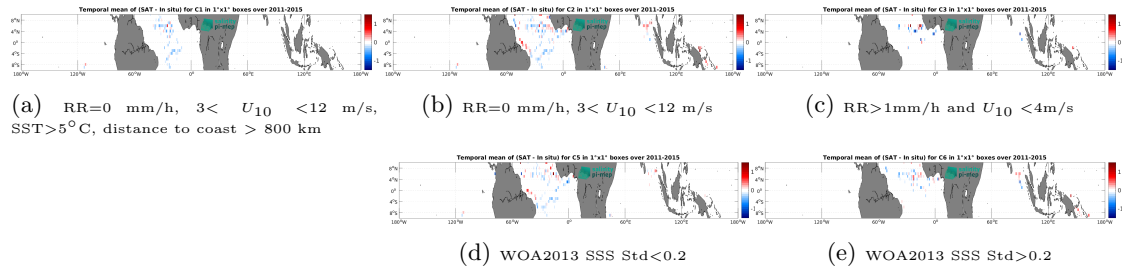
Figure 11: Temporal mean gridded over spatial boxes of size 1^\circ \times 1^\circ of \Delta SSS (Aquarius SSS L2 OR v5 (NASA-GSFC) - Surface drifters) for 5 different subdatasets corresponding to: RR=0 mm/h, 3 < U_{10} < 12 m/s, SST >5^\circ C, distance to coast > 800 km (a), RR=0 mm/h, 3 < U_{10} < 12 m/s (b), RR >1 mm/h and U_{10} < 4 m/s (c), WOA2013 SSS Std <0.2 (d), WOA2013 SSS Std >0.2 (e).
