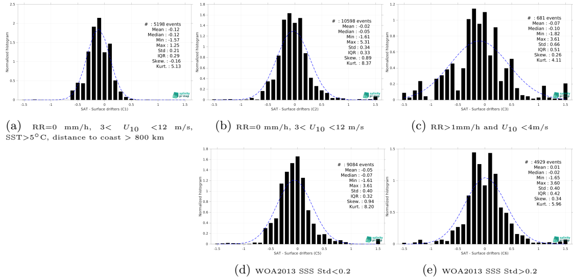
Figure 12: Normalized histogram of \Delta SSS (Aquarius SSS L2 OR v5 (NASA-GSFC) - Surface drifters) for 5 different subdatasets corresponding to: RR=0 mm/h, 3 < U_{10} < 12 m/s, SST >5^\circ C, distance to coast > 800 km (a), RR=0 mm/h, 3 < U_{10} < 12 m/s (b), RR >1 mm/h and U_{10} < 4 m/s (c), WOA2013 SSS Std <0.2 (d), WOA2013 SSS Std >0.2 (e).
