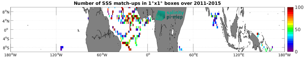
Figure 3: Number of SSS match-ups between Surface drifters SSS and the Aquarius SSS L2 OR v5 (NASA-GSFC) SSS product for the Equatorial Ocean 10N-10S Pi-MEP region over 1^\circ \times 1^\circ boxes and for the full satellite product period.
