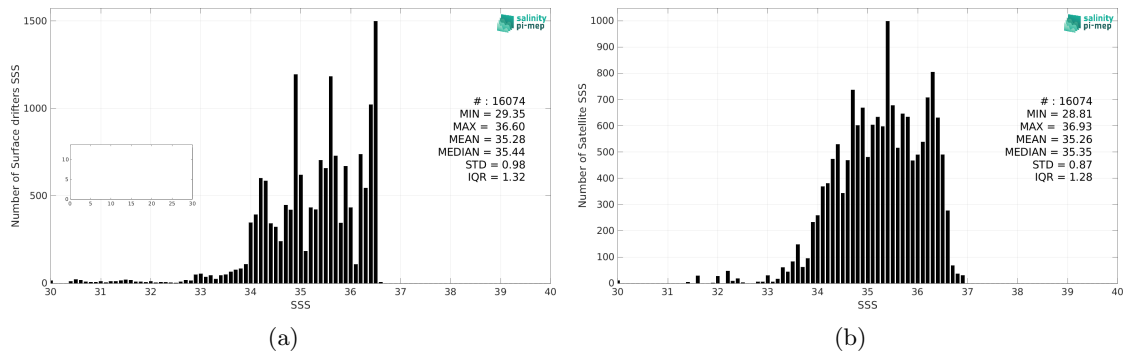
Figure 2: Histograms of SSS from Surface drifters (a) and Aquarius SSS L2 OR v5 (NASA-GSFC) (b) considering all match-up pairs per bins of 0.1 over the Equatorial Ocean 10N-10S Pi-MEP region and for the full satellite product period.
