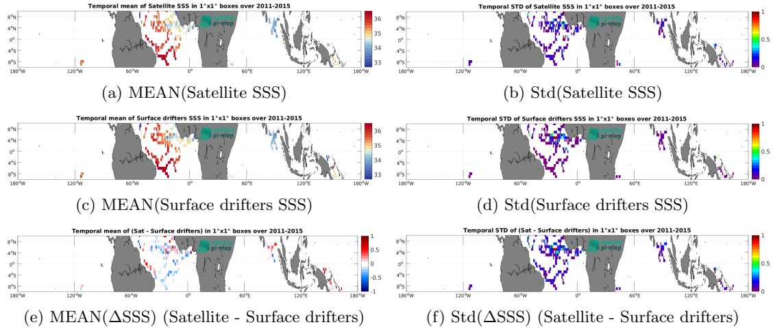
Figure 5: Temporal mean (left) and Std (right) of SSS from Aquarius SSS L2 OR v5 (NASA-GSFC) (top), Surface drifters (middle), and of \Delta SSS (Satellite - Surface drifters). Only match-up pairs are used to generate these maps.
