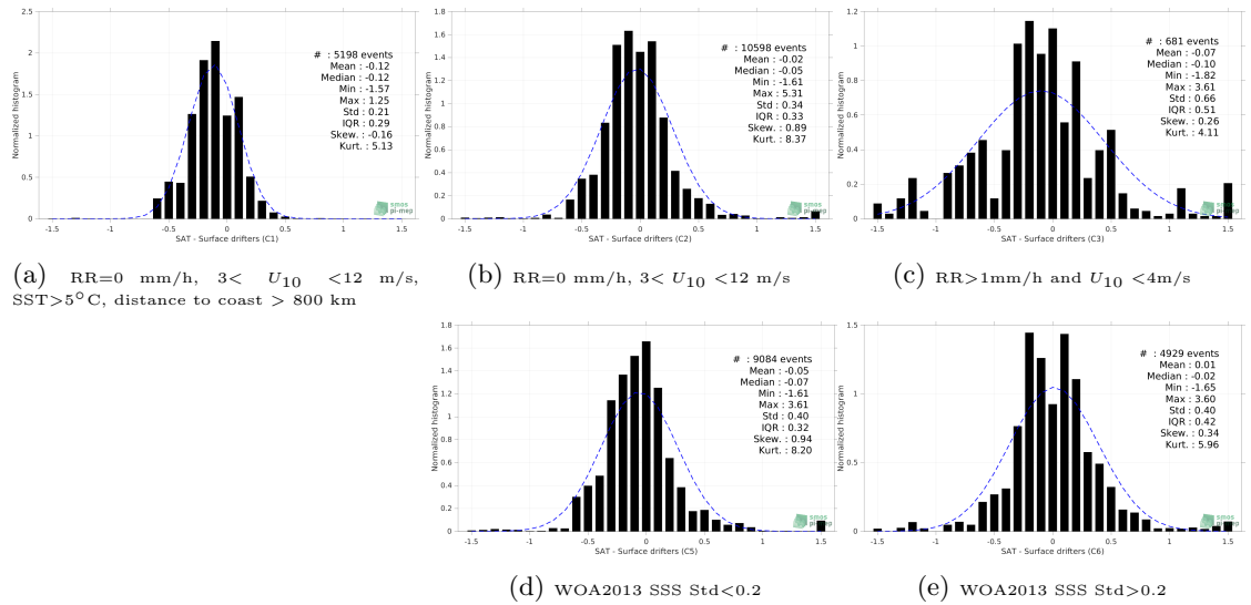
Figure 12: Normalized histogram of \Delta SSS (Aquarius SSS L2 OR v5 (NASA-GSFC) - Surface drifters) for 5 different subdatasets corresponding to: RR=0 mm/h, 3 < U_{10} < 12 m/s, SST > 5^\circ C , distance to coast > 800 km (a), RR=0 mm/h, 3 < U_{10} < 12 m/s (b), RR>1mm/h and U_{10} < 4 m/s (c), WOA2013 SSS Std<0.2 (d), WOA2013 SSS Std>0.2 (e).
