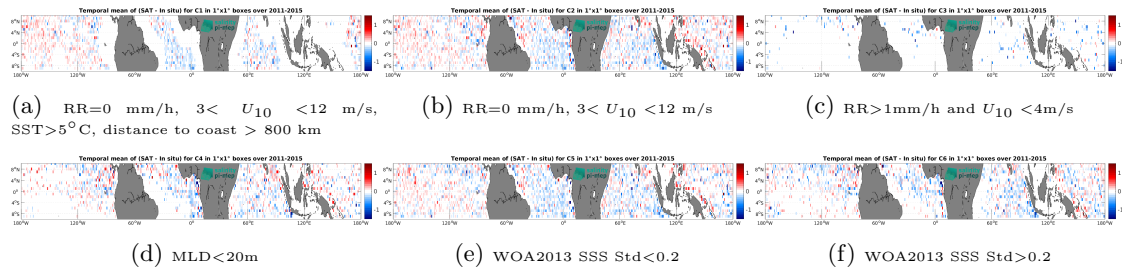
Figure 14: Temporal mean gridded over spatial boxes of size 1^\circ \times 1^\circ of \Delta SSS (Aquarius SSS L2 OR v5 (NASA-GSFC) - Argo) for 6 different subdatasets corresponding to:RR=0 mm/h, 3 < U_{10} < 12 m/s, SST >5^\circ C, distance to coast > 800 km (a), RR=0 mm/h, 3 < U_{10} < 12 m/s (b), RR >1 mm/h and U_{10} < 4 m/s (c),MLD <20 m (d),WOA2013 SSS Std <0.2 (e),WOA2013 SSS Std >0.2 (f).
