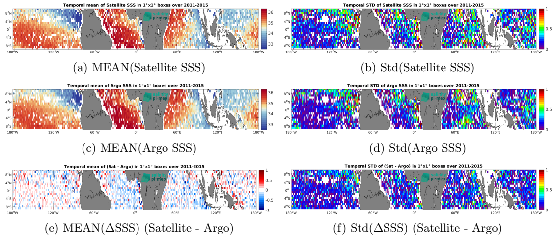
Figure 7: Temporal mean (left) and Std (right) of SSS from Aquarius SSS L2 OR v5 (NASA-GSFC) (top), Argo (middle), and of \Delta SSS (Satellite - Argo). Only match-up pairs are used to generate these maps.
