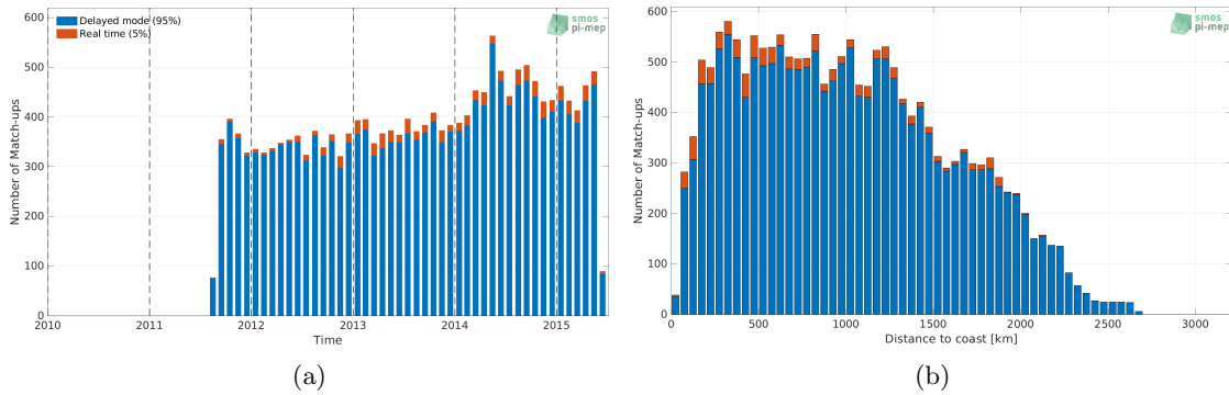
Figure 1: Number of match-ups between Argo and Aquarius SSS L2 OR v5 (NASA-GSFC) SSS as a function of time (a) and as function of the distance to coast (b) over the Equatorial Ocean 10N-10S Pi-MEP region and for the full satellite product period.
