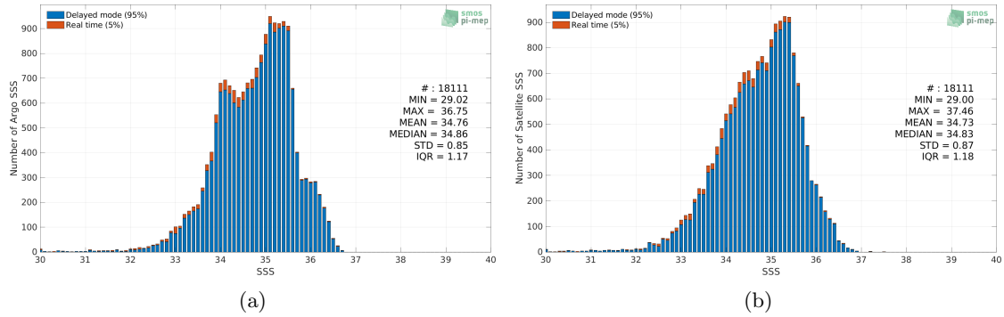
Figure 2: Histograms of SSS from Argo (a) and Aquarius SSS L2 OR v5 (NASA-GSFC) (b) considering all match-up pairs per bins of 0.1 over the Equatorial Ocean 10N-10S Pi-MEP region and for the full satellite product period.
