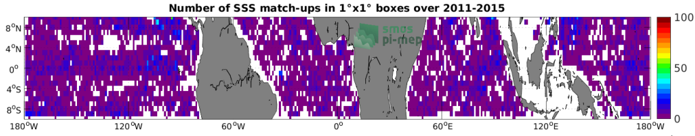
Figure 4: Number of SSS match-ups between Argo SSS and the Aquarius SSS L2 OR v5 (NASA-GSFC) SSS product for the Equatorial Ocean 10N-10S Pi-MEP region over 1^\circ \times 1^\circ boxes and for the full satellite product period.
