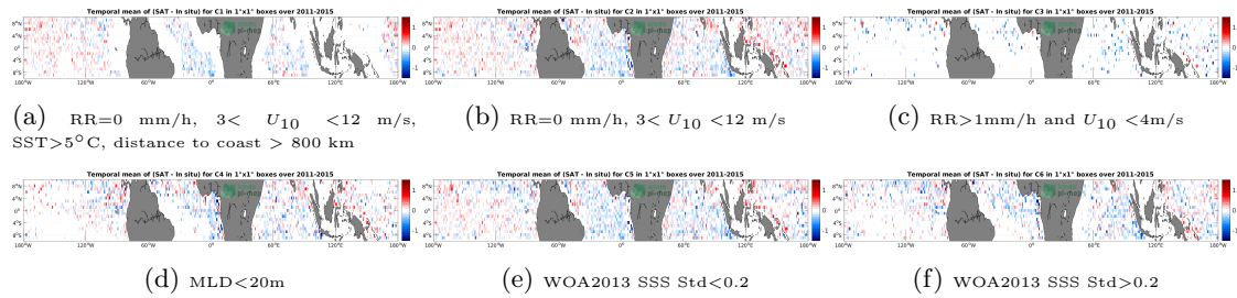
Figure 12: Temporal mean gridded over spatial boxes of size 1^\circ \times 1^\circ of \Delta SSS (Aquarius SSS L2 OR v5 (NASA-GSFC) - Argo) for 6 different subdatasets corresponding to:RR=0 mm/h, 3 < U_{10} < 12 m/s, SST >5^\circ\text{C} , distance to coast > 800 km (a), RR=0 mm/h, 3 < U_{10} < 12 m/s (b), RR >1 mm/h and U_{10} < 4 m/s (c),MLD <20 m (d),WOA2013 SSS Std <0.2 (e),WOA2013 SSS Std >0.2 (f).
