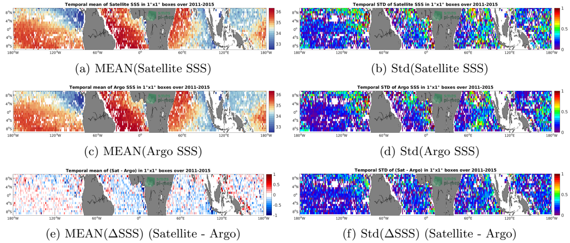
Figure 6: Temporal mean (left) and Std (right) of SSS from Aquarius SSS L2 OR v5 (NASA-GSFC) (top), Argo (middle), and of \Delta SSS (Satellite - Argo). Only match-up pairs are used to generate these maps.
