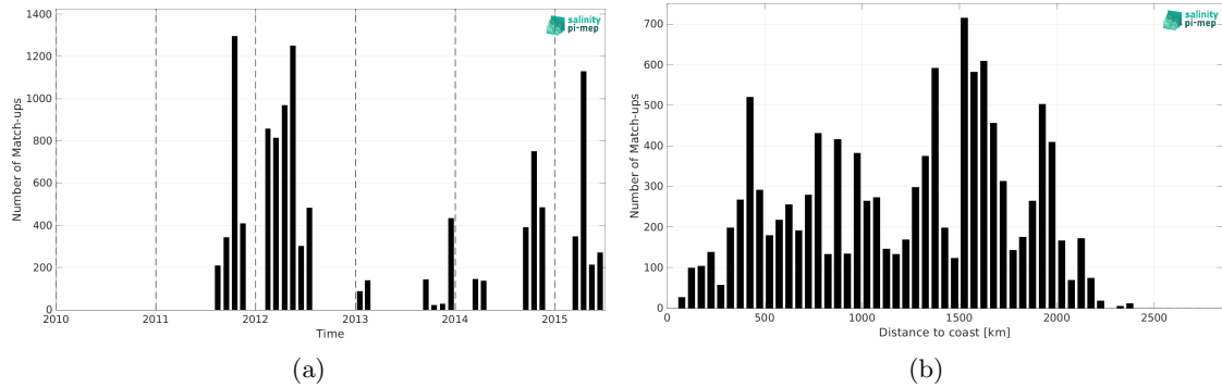
Figure 2: Number of match-ups between TSG (SAMOS) and Aquarius SSS L2 CAP v5 (JPL) SSS as a function of time (a) and as function of the distance to coast (b) over the Equatorial Ocean 10N-10S Pi-MEP region and for the full satellite product period.
