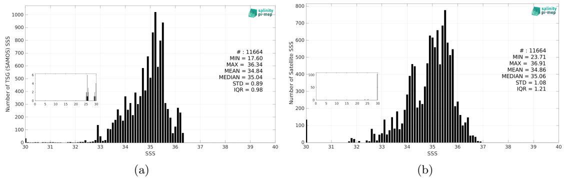
Figure 3: Histograms of SSS from TSG (SAMOS) (a) and Aquarius SSS L2 CAP v5 (JPL) (b) considering all match-up pairs per bins of 0.1 over the Equatorial Ocean 10N-10S Pi-MEP region and for the full satellite product period.
