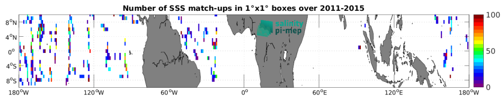
Figure 5: Number of SSS match-ups between TSG (SAMOS) SSS and the Aquarius SSS L2 CAP v5 (JPL) SSS product for the Equatorial Ocean 10N-10S Pi-MEP region over 1^\circ \times 1^\circ boxes and for the full satellite product period.
