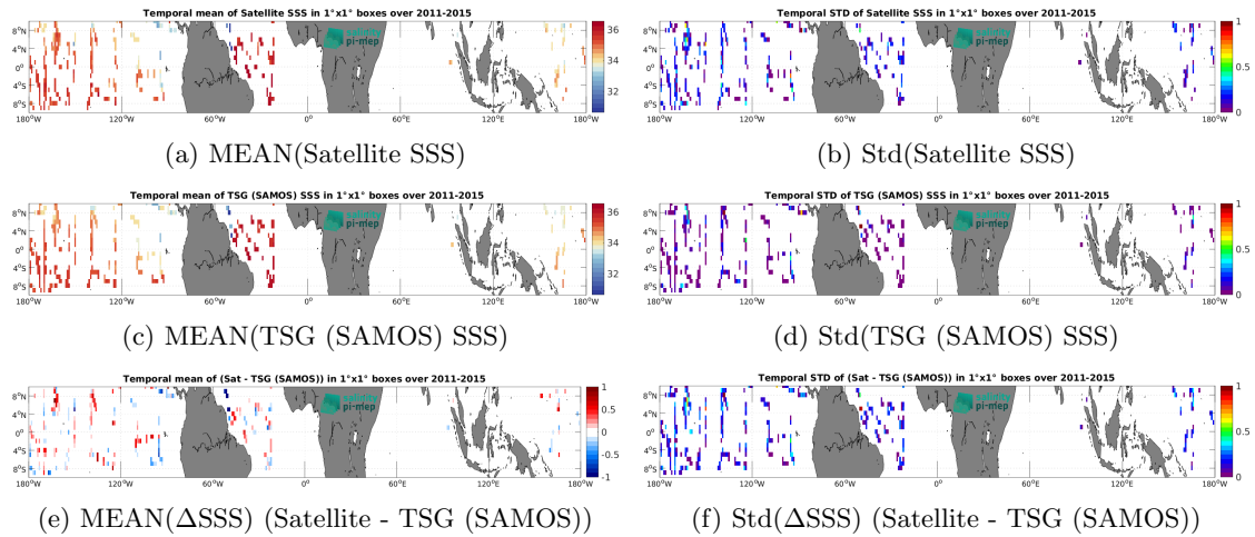
Figure 7: Temporal mean (left) and Std (right) of SSS from Aquarius SSS L2 CAP v5 (JPL) (top), TSG (SAMOS) (middle), and of \Delta SSS (Satellite - TSG (SAMOS)). Only match-up pairs are used to generate these maps.
