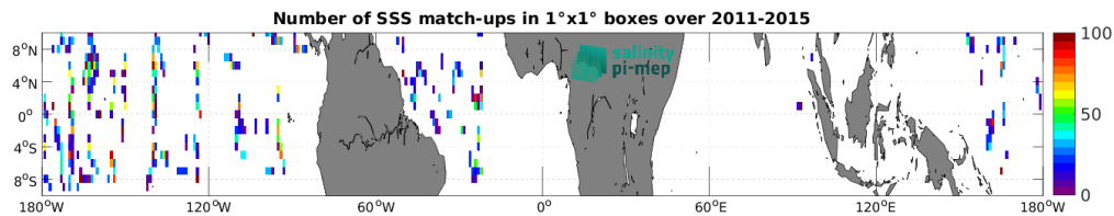
Figure 5: Number of SSS match-ups between TSG (SAMOS) SSS and the Aquarius SSS L2 CAP v5 (JPL) SSS product for the Equatorial Ocean 10N-10S Pi-MEP region over 1^\circ \times 1^\circ boxes and for the full satellite product period.
