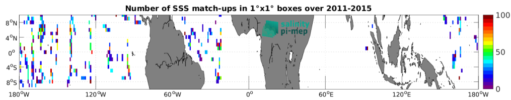
Figure 4: Number of SSS match-ups between TSG (SAMOS) SSS and the Aquarius SSS L2 CAP v5 (JPL) SSS product for the Equatorial Ocean 10N-10S Pi-MEP region over 1^\circ \times 1^\circ boxes and for the full satellite product period.
