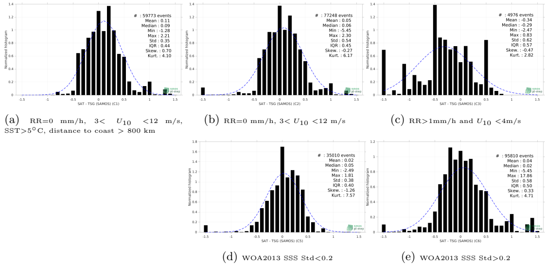
Figure 13: Normalized histogram of \Delta SSS (Aquarius SSS L2 CAP v5 (JPL) - TSG (SAMOS)) for 5 different subdatasets corresponding to: RR=0 mm/h, 3 < U_{10} < 12 m/s, SST >5^\circ\text{C} , distance to coast > 800 km (a), RR=0 mm/h, 3 < U_{10} < 12 m/s (b), RR >1 mm/h and U_{10} < 4 m/s (c), WOA2013 SSS Std <0.2 (d), WOA2013 SSS Std >0.2 (e).
