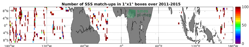
Figure 4: Number of SSS match-ups between TSG-SAMOS SSS and the Aquarius-L2-JPL-V5 SSS product for the Equatorial Ocean 10N-10S Pi-MEP region over 1^\circ \times 1^\circ boxes and for the full satellite product period.
