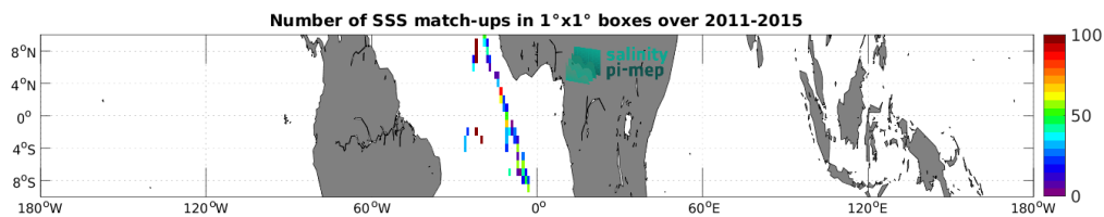
Figure 4: Number of SSS match-ups between TSG (Polarstern) SSS and the Aquarius SSS L2 CAP v5 (JPL) SSS product for the Equatorial Ocean 10N-10S Pi-MEP region over 1^\circ \times 1^\circ boxes and for the full satellite product period.
