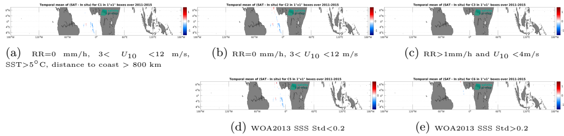
Figure 12: Temporal mean gridded over spatial boxes of size 1^\circ \times 1^\circ of \Delta\text{SSS} (Aquarius SSS L2 CAP v5 (JPL) - TSG (Polarstern)) for 5 different subdatasets corresponding to:RR=0 mm/h, 3 < U_{10} < 12 m/s, SST >5^\circ\text{C} , distance to coast > 800 km (a), RR=0 mm/h, 3 < U_{10} < 12 m/s (b), RR >1 mm/h and U_{10} < 4 m/s (c), WOA2013 SSS Std <0.2 (d), WOA2013 SSS Std >0.2 (e).
