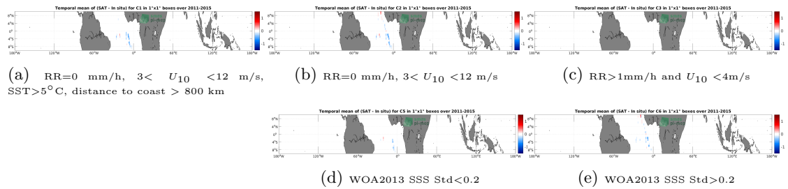
Figure 12: Temporal mean gridded over spatial boxes of size 1^\circ \times 1^\circ of \Delta SSS (Aquarius SSS L2 CAP v5 (JPL) - TSG (Polarstern)) for 5 different subdatasets corresponding to:RR=0 mm/h, 3 < U_{10} < 12 m/s, SST > 5^\circ C , distance to coast > 800 km (a), RR=0 mm/h, 3 < U_{10} < 12 m/s (b), RR>1mm/h and U_{10} < 4 m/s (c), WOA2013 SSS Std<0.2 (d), WOA2013 SSS Std>0.2 (e).
