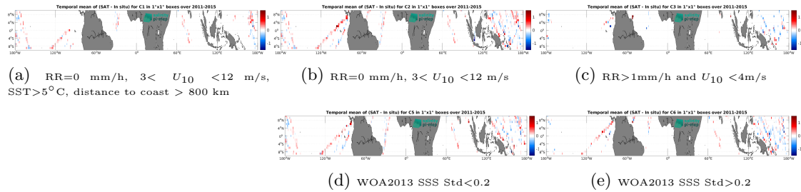
Figure 12: Temporal mean gridded over spatial boxes of size 1^\circ \times 1^\circ of \Delta\text{SSS} (Aquarius SSS L2 CAP v5 (JPL) - TSG (LEGOS-DM)) for 5 different subdatasets corresponding to:RR=0 mm/h, 3 < U_{10} < 12 m/s, SST >5^\circ\text{C} , distance to coast > 800 km (a), RR=0 mm/h, 3 < U_{10} < 12 m/s (b), RR >1 mm/h and U_{10} < 4 m/s (c), WOA2013 SSS Std <0.2 (d), WOA2013 SSS Std >0.2 (e).
