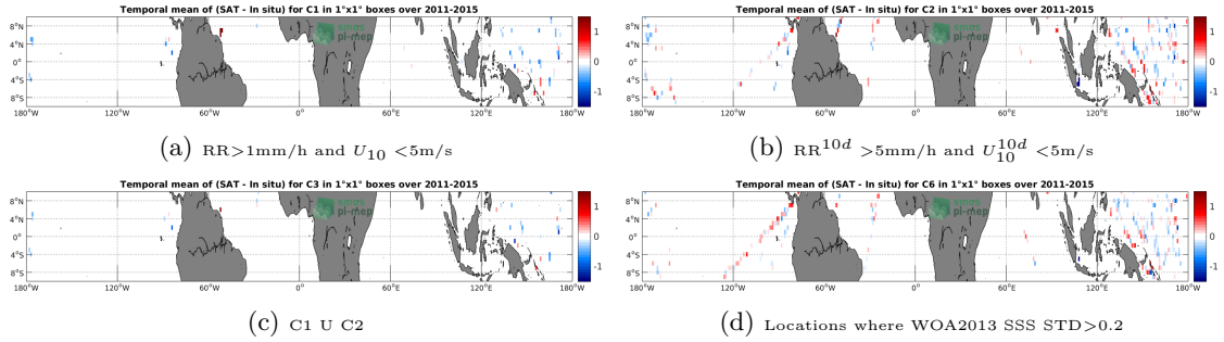
Figure 12: Temporal mean gridded over spatial boxes of size 1^\circ \times 1^\circ of \Delta SSS (Aquarius-L2-JPL-V5 - TSG-LEGOS-DM) for 4 different subdatasets corresponding to: RR >1 mm/h and U_{10} < 5 m/s (a), RR ^{10d} > 5 mm/h and U_{10}^{10d} < 5 m/s (b), C1 U C2 (c), Locations where WOA2013 SSS STD >0.2 (d).
