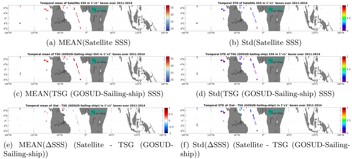
Figure 7: Temporal mean (left) and Std (right) of SSS from Aquarius SSS L2 CAP v5 (JPL) (top), TSG (GOSUD-Sailing-ship) (middle), and of \Delta SSS (Satellite - TSG (GOSUD-Sailing-ship)). Only match-up pairs are used to generate these maps.
