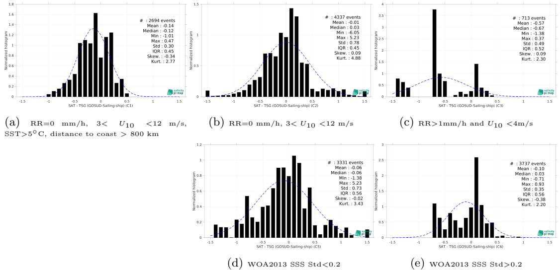
Figure 15: Normalized histogram of \Delta\text{SSS} (Aquarius SSS L2 CAP v5 (JPL) - TSG (GOSUD-Sailing-ship)) for 5 different subdatasets corresponding to: RR=0 mm/h, 3 < U_{10} < 12 m/s, SST>5°C, distance to coast > 800 km (a), RR=0 mm/h, 3 < U_{10} < 12 m/s (b), RR>1mm/h and U_{10} < 4 m/s (c), WOA2013 SSS Std<0.2 (d), WOA2013 SSS Std>0.2 (e).
