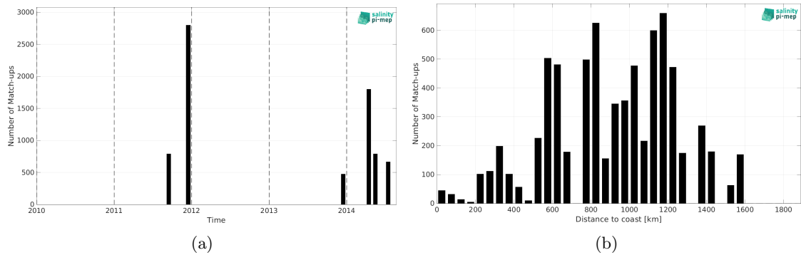
Figure 2: Number of match-ups between TSG (GOSUD-Sailing-ship) and Aquarius SSS L2 CAP v5 (JPL) SSS as a function of time (a) and as function of the distance to coast (b) over the Equatorial Ocean 10N-10S Pi-MEP region and for the full satellite product period.
