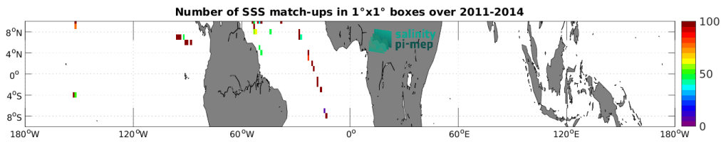
Figure 5: Number of SSS match-ups between TSG (GOSUD-Sailing-ship) SSS and the Aquarius SSS L2 CAP v5 (JPL) SSS product for the Equatorial Ocean 10N-10S Pi-MEP region over 1^\circ \times 1^\circ boxes and for the full satellite product period.
