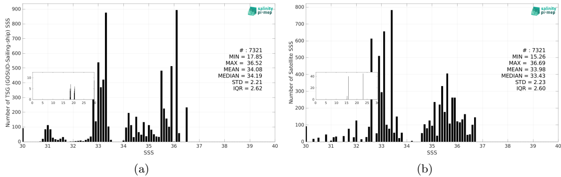
Figure 3: Histograms of SSS from TSG (GOSUD-Sailing-ship) (a) and Aquarius SSS L2 CAP v5 (JPL) (b) considering all match-up pairs per bins of 0.1 over the Equatorial Ocean 10N-10S Pi-MEP region and for the full satellite product period.
