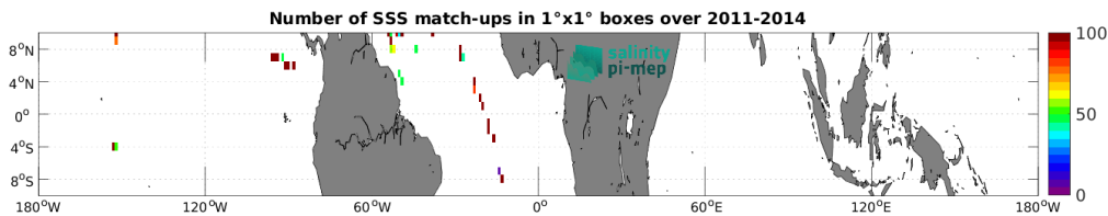
Figure 5: Number of SSS match-ups between TSG (GOSUD-Sailing-ship) SSS and the Aquarius SSS L2 CAP v5 (JPL) SSS product for the Equatorial Ocean 10N-10S Pi-MEP region over 1^\circ \times 1^\circ boxes and for the full satellite product period.
