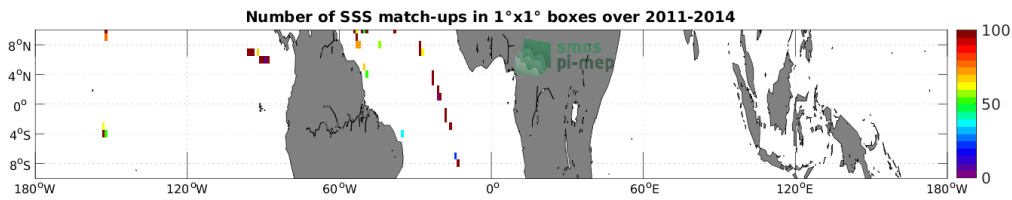
Figure 4: Number of SSS match-ups between TSG (GOSUD-Sailing-ship) SSS and the Aquarius SSS L2 CAP v5 (JPL) SSS product for the Equatorial Ocean 10N-10S Pi-MEP region over 1^\circ \times 1^\circ boxes and for the full satellite product period.
