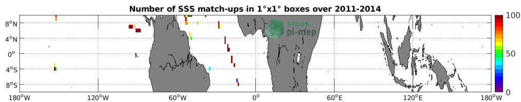
Figure 4: Number of SSS match-ups between TSG (GOSUD-Sailing-ship) SSS and the Aquarius SSS L2 CAP v5 (JPL) SSS product for the Equatorial Ocean 10N-10S Pi-MEP region over 1^\circ \times 1^\circ boxes and for the full satellite product period.
