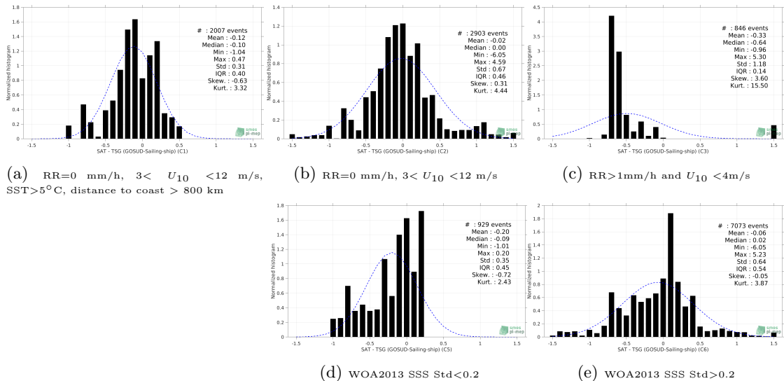
Figure 13: Normalized histogram of \Delta SSS (Aquarius SSS L2 CAP v5 (JPL) - TSG (GOSUD-Sailing-ship)) for 5 different subdatasets corresponding to: RR=0 mm/h, 3 < U_{10} < 12 m/s, SST> 5^\circ C , distance to coast > 800 km (a), RR=0 mm/h, 3 < U_{10} < 12 m/s (b), RR>1mm/h and U_{10} < 4 m/s (c), WOA2013 SSS Std<0.2 (d), WOA2013 SSS Std>0.2 (e).
