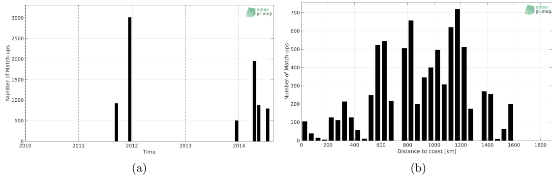
Figure 1: Number of match-ups between TSG (GOSUD-Sailing-ship) and Aquarius SSS L2 CAP v5 (JPL) SSS as a function of time (a) and as function of the distance to coast (b) over the Equatorial Ocean 10N-10S Pi-MEP region and for the full satellite product period.
