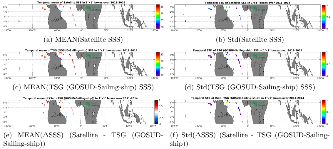
Figure 6: Temporal mean (left) and Std (right) of SSS from Aquarius SSS L2 CAP v5 (JPL) (top), TSG (GOSUD-Sailing-ship) (middle), and of \Delta SSS (Satellite - TSG (GOSUD-Sailing-ship)). Only match-up pairs are used to generate these maps.
