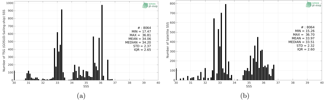
Figure 2: Histograms of SSS from TSG (GOSUD-Sailing-ship) (a) and Aquarius SSS L2 CAP v5 (JPL) (b) considering all match-up pairs per bins of 0.1 over the Equatorial Ocean 10N-10S Pi-MEP region and for the full satellite product period.
