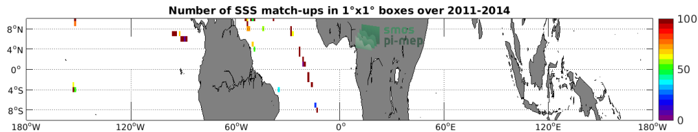
Figure 4: Number of SSS match-ups between TSG (GOSUD-Sailing-ship) SSS and the Aquarius SSS L2 CAP v5 (JPL) SSS product for the Equatorial Ocean 10N-10S Pi-MEP region over 1°x1° boxes and for the full satellite product period.
