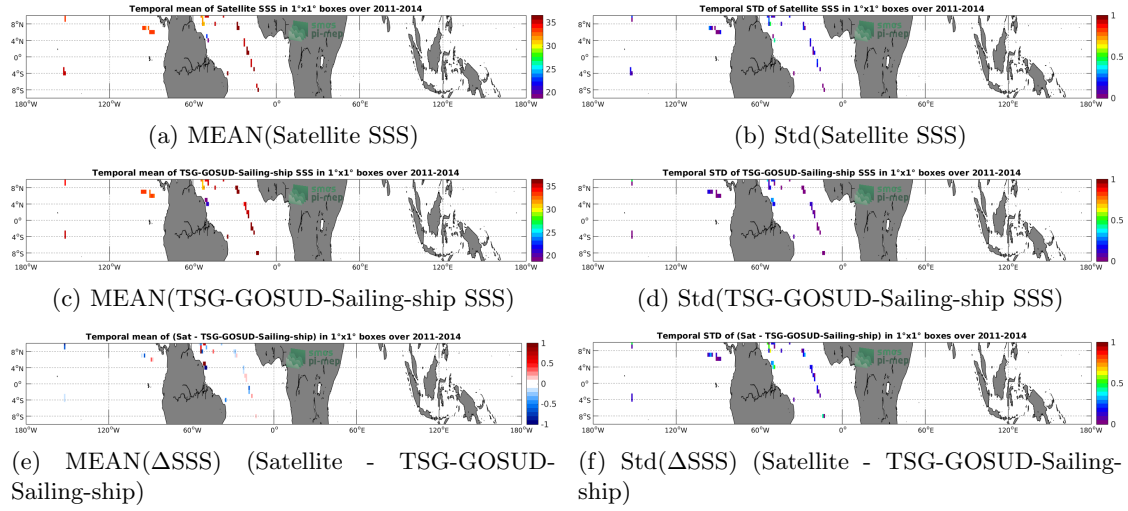
Figure 6: Temporal mean (left) and Std (right) of SSS from Aquarius-L2-JPL-V5 (top), TSG-GOSUD-Sailing-ship (middle), and of \Delta SSS (Satellite - TSG-GOSUD-Sailing-ship). Only match-up pairs are used to generate these maps.
