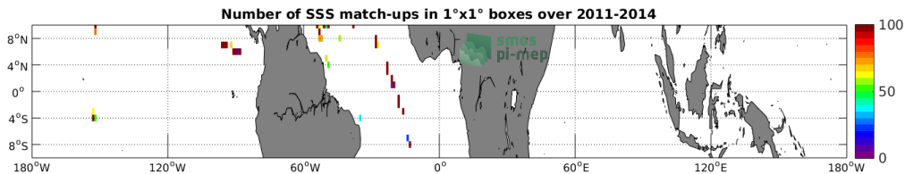
Figure 4: Number of SSS match-ups between TSG-GOSUD-Sailing-ship SSS and the Aquarius-L2-JPL-V5 SSS product for the Equatorial Ocean 10N-10S Pi-MEP region over 1°x1° boxes and for the full satellite product period.
