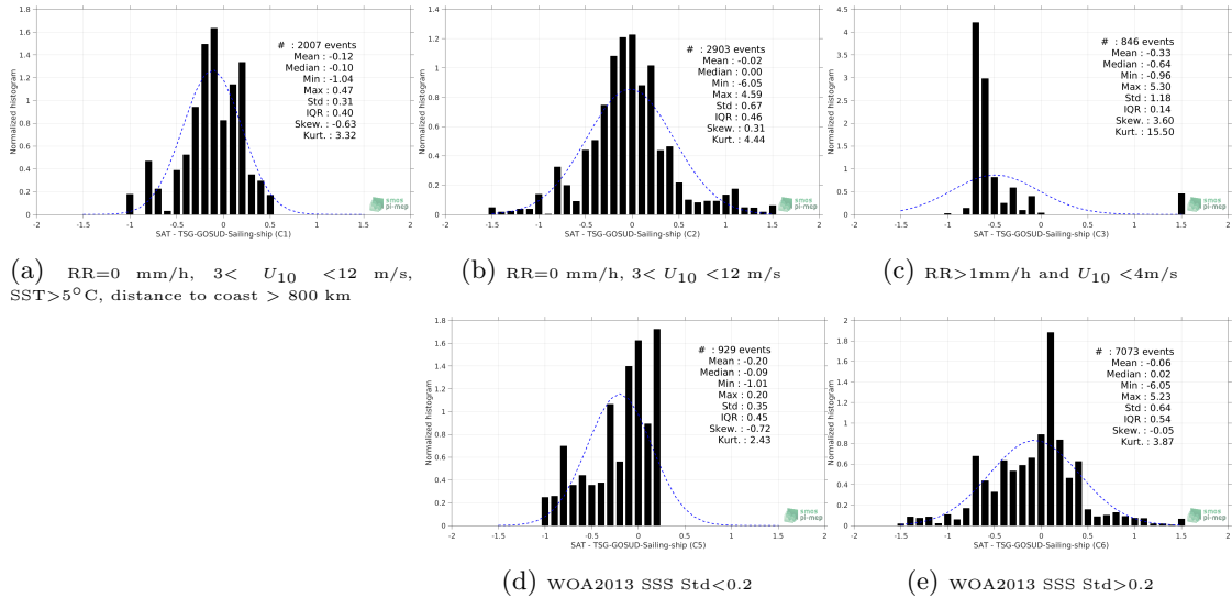
Figure 13: Normalized histogram of ΔSSS (Aquarius-L2-JPL-V5 - TSG-GOSUD-Sailing-ship) for 5 different subdatasets corresponding to: RR=0 mm/h, 3 < U 10 < 12 m/s, SST > 5°C, distance to coast > 800 km (a), RR=0 mm/h, 3 < U 10 < 12 m/s (b), RR > 1mm/h and U 10 < 4m/s (c), WOA2013 SSS Std < 0.2 (d), WOA2013 SSS Std > 0.2 (e).
