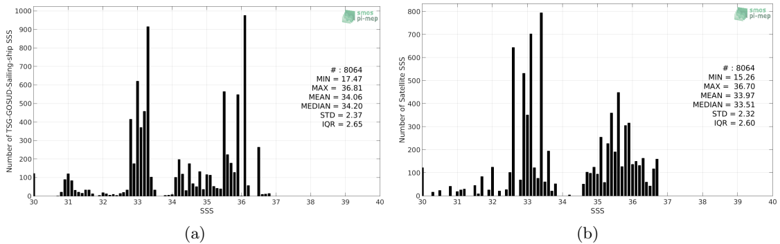
Figure 2: Histograms of SSS from TSG-GOSUD-Sailing-ship (a) and Aquarius-L2-JPL-V5 (b) considering all match-up pairs per bins of 0.1 over the Equatorial Ocean 10N-10S Pi-MEP region and for the full satellite product period.
