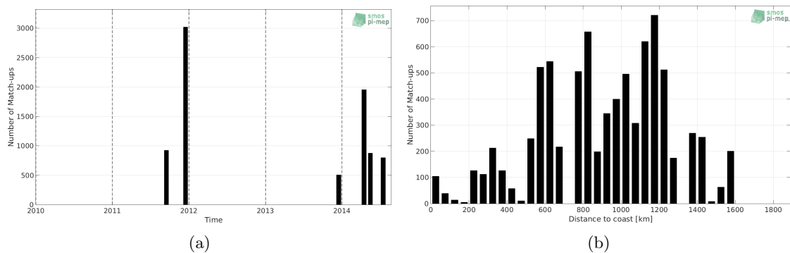
Figure 1: Number of match-ups between TSG-GOSUD-Sailing-ship and Aquarius-L2-JPL-V5 SSS as a function of time (a) and as function of the distance to coast (b) over the Equatorial Ocean 10N-10S Pi-MEP region and for the full satellite product period.
