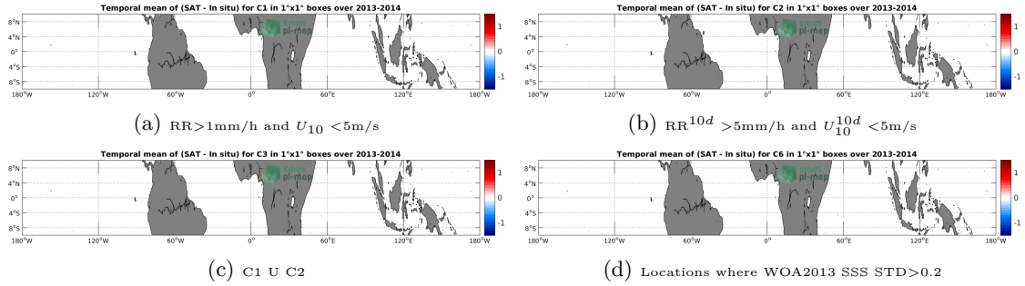
Figure 12: Temporal mean gridded over spatial boxes of size 1^\circ \times 1^\circ of \Delta SSS (Aquarius-L2-JPL-V5 - TSG-GOSUD-Sailing-ship) for 4 different subdatasets corresponding to: RR>1mm/h and U_{10} < 5m/s (a), RR^{10d} > 5mm/h and U_{10}^{10d} < 5m/s (b), C1 U C2 (c), Locations where WOA2013 SSS STD>0.2 (d).
