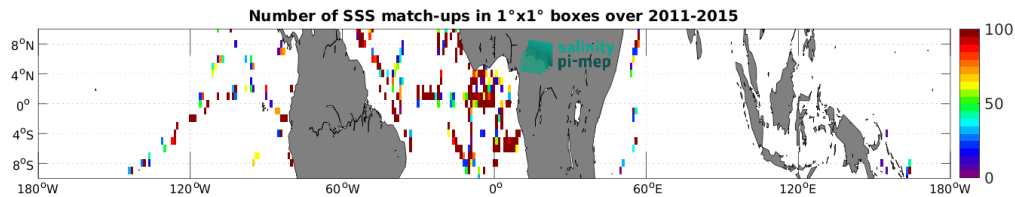
Figure 5: Number of SSS match-ups between TSG (GOSUD-Research-vessel) SSS and the Aquarius SSS L2 CAP v5 (JPL) SSS product for the Equatorial Ocean 10N-10S Pi-MEP region over 1^\circ \times 1^\circ boxes and for the full satellite product period.
