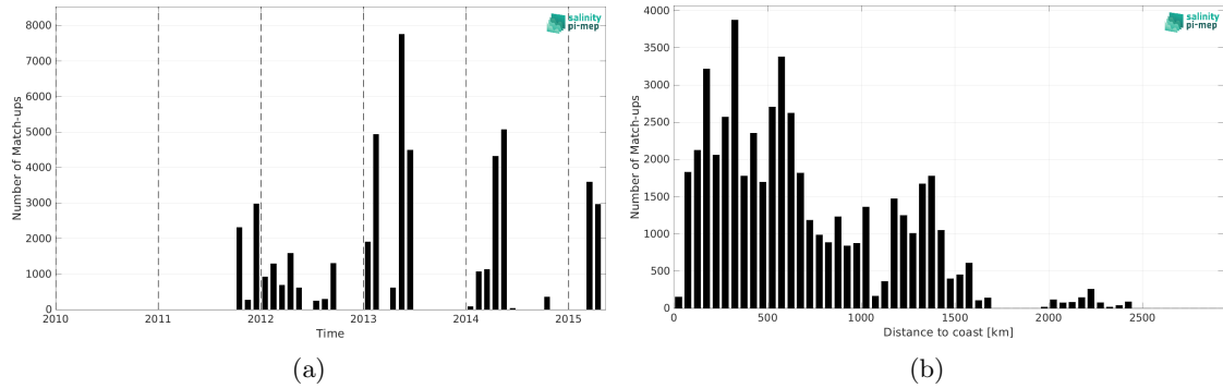
Figure 2: Number of match-ups between TSG (GOSUD-Research-vessel) and Aquarius SSS L2 CAP v5 (JPL) SSS as a function of time (a) and as function of the distance to coast (b) over the Equatorial Ocean 10N-10S Pi-MEP region and for the full satellite product period.
