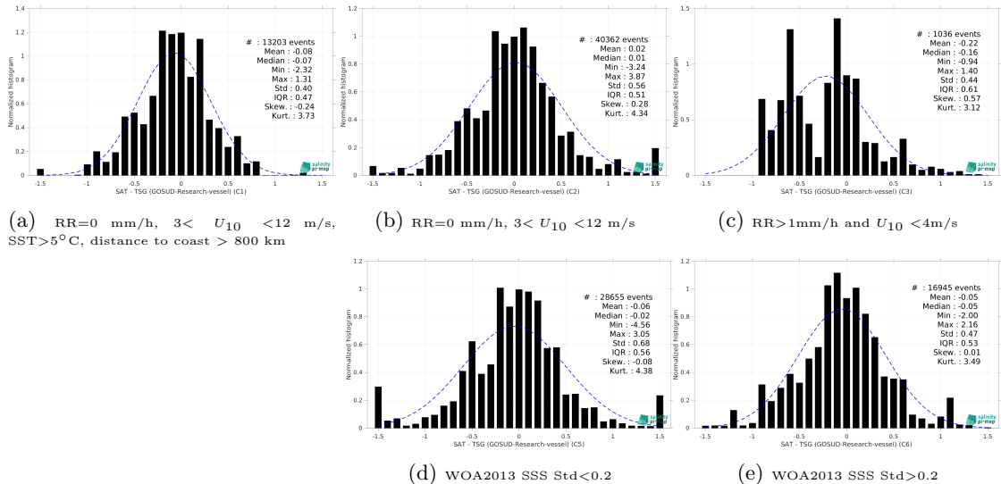
Figure 15: Normalized histogram of \Delta SSS (Aquarius SSS L2 CAP v5 (JPL) - TSG (GOSUD-Research-vessel)) for 5 different subdatasets corresponding to: RR=0 mm/h, 3 < U_{10} < 12 m/s, SST >5^\circ C, distance to coast > 800 km (a), RR=0 mm/h, 3 < U_{10} < 12 m/s (b), RR >1 mm/h and U_{10} < 4 m/s (c), WOA2013 SSS Std <0.2 (d), WOA2013 SSS Std >0.2 (e).
