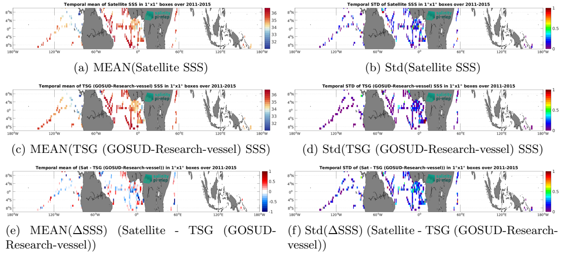
Figure 7: Temporal mean (left) and Std (right) of SSS from Aquarius SSS L2 CAP v5 (JPL) (top), TSG (GOSUD-Research-vessel) (middle), and of \Delta SSS (Satellite - TSG (GOSUD-Research-vessel)). Only match-up pairs are used to generate these maps.
