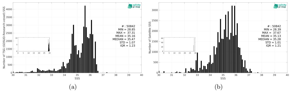
Figure 3: Histograms of SSS from TSG (GOSUD-Research-vessel) (a) and Aquarius SSS L2 CAP v5 (JPL) (b) considering all match-up pairs per bins of 0.1 over the Equatorial Ocean 10N-10S Pi-MEP region and for the full satellite product period.
