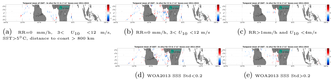
Figure 14: Temporal mean gridded over spatial boxes of size 1^\circ \times 1^\circ of \Delta SSS (Aquarius SSS L2 CAP v5 (JPL) - TSG (GOSUD-Research-vessel)) for 5 different subdatasets corresponding to: RR=0 mm/h, 3 < U_{10} < 12 m/s, SST >5^\circ C, distance to coast > 800 km (a), RR=0 mm/h, 3 < U_{10} < 12 m/s (b), RR >1 mm/h and U_{10} < 4 m/s (c), WOA2013 SSS Std <0.2 (d), WOA2013 SSS Std >0.2 (e).
