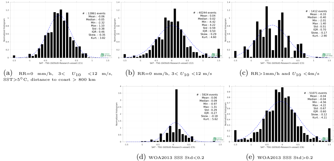
Figure 13: Normalized histogram of \Delta\text{SSS} (Aquarius SSS L2 CAP v5 (JPL) - TSG (GOSUD-Research-vessel)) for 5 different subdatasets corresponding to: RR=0 mm/h, 3 < U_{10} < 12 m/s, SST>5°C, distance to coast > 800 km (a), RR=0 mm/h, 3 < U_{10} < 12 m/s (b), RR>1mm/h and U_{10} < 4 m/s (c), WOA2013 SSS Std<0.2 (d), WOA2013 SSS Std>0.2 (e).
