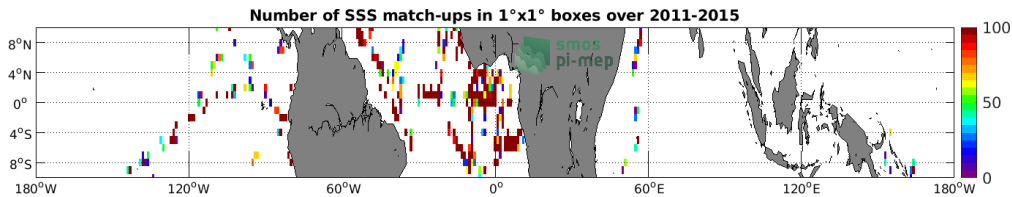
Figure 4: Number of SSS match-ups between TSG (GOSUD-Research-vessel) SSS and the Aquarius SSS L2 CAP v5 (JPL) SSS product for the Equatorial Ocean 10N-10S Pi-MEP region over 1^\circ \times 1^\circ boxes and for the full satellite product period.
