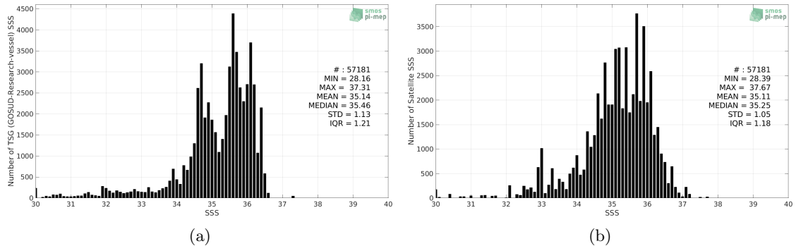
Figure 2: Histograms of SSS from TSG (GOSUD-Research-vessel) (a) and Aquarius SSS L2 CAP v5 (JPL) (b) considering all match-up pairs per bins of 0.1 over the Equatorial Ocean 10N-10S Pi-MEP region and for the full satellite product period.
