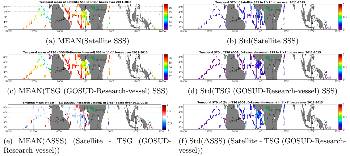
Figure 6: Temporal mean (left) and Std (right) of SSS from Aquarius SSS L2 CAP v5 (JPL) (top), TSG (GOSUD-Research-vessel) (middle), and of \Delta SSS (Satellite - TSG (GOSUD-Research-vessel)). Only match-up pairs are used to generate these maps.
