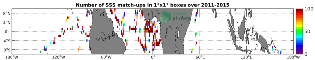
Figure 4: Number of SSS match-ups between TSG (GOSUD-Research-vessel) SSS and the Aquarius SSS L2 CAP v5 (JPL) SSS product for the Equatorial Ocean 10N-10S Pi-MEP region over 1°x1° boxes and for the full satellite product period.
