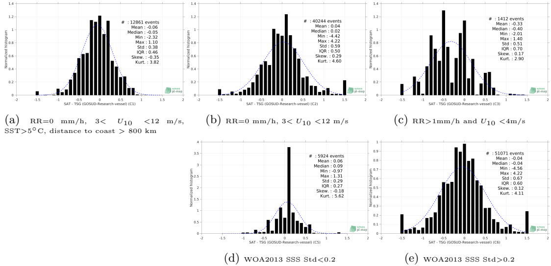
Figure 13: Normalized histogram of \Delta SSS (Aquarius SSS L2 CAP v5 (JPL) - TSG (GOSUD-Research-vessel)) for 5 different subdatasets corresponding to: RR=0 mm/h, 3 < U_{10} < 12 m/s, SST > 5^\circ C , distance to coast > 800 km (a), RR=0 mm/h, 3 < U_{10} < 12 m/s (b), RR > 1 mm/h and U_{10} < 4 m/s (c), WOA2013 SSS Std < 0.2 (d), WOA2013 SSS Std > 0.2 (e).
