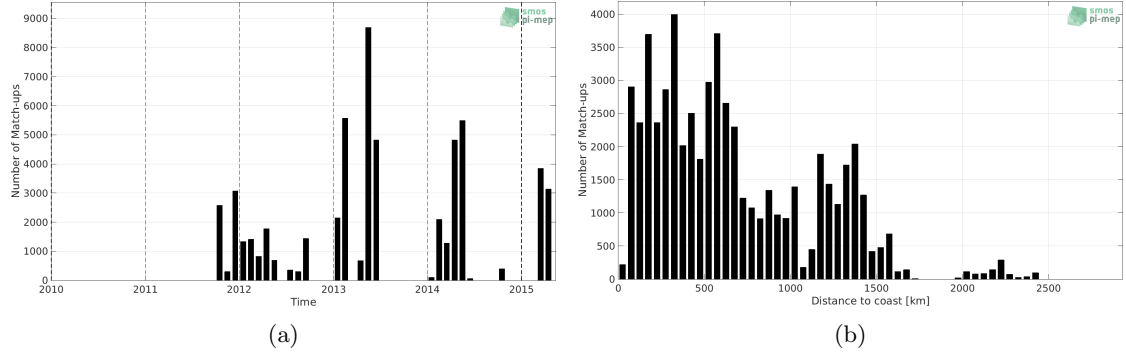
Figure 1: Number of match-ups between TSG (GOSUD-Research-vessel) and Aquarius SSS L2 CAP v5 (JPL) SSS as a function of time (a) and as function of the distance to coast (b) over the Equatorial Ocean 10N-10S Pi-MEP region and for the full satellite product period.
