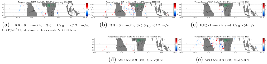
Figure 12: Temporal mean gridded over spatial boxes of size 1^\circ \times 1^\circ of \Delta SSS (Aquarius SSS L2 CAP v5 (JPL) - TSG (GOSUD-Research-vessel)) for 5 different subdatasets corresponding to: RR=0 mm/h, 3 < U_{10} < 12 m/s, SST > 5^\circ C , distance to coast > 800 km (a), RR=0 mm/h, 3 < U_{10} < 12 m/s (b), RR > 1 mm/h and U_{10} < 4 m/s (c), WOA2013 SSS Std < 0.2 (d), WOA2013 SSS Std > 0.2 (e).
