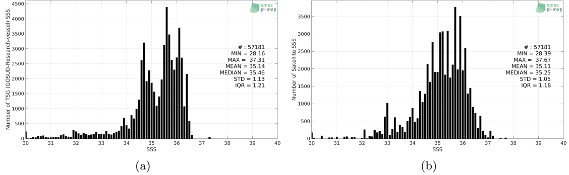
Figure 2: Histograms of SSS from TSG (GOSUD-Research-vessel) (a) and Aquarius SSS L2 CAP v5 (JPL) (b) considering all match-up pairs per bins of 0.1 over the Equatorial Ocean 10N-10S Pi-MEP region and for the full satellite product period.
