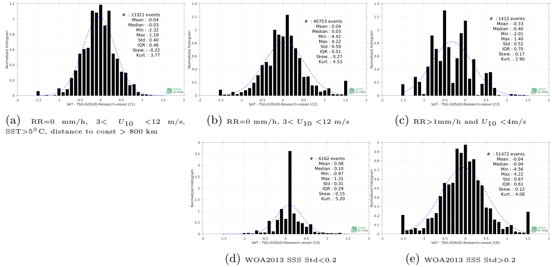
Figure 13: Normalized histogram of \Delta SSS (Aquarius-L2-JPL-V5 - TSG-GOSUD-Research-vessel) for 5 different subdatasets corresponding to: RR=0 mm/h, 3 < U_{10} < 12 m/s, SST >5^\circ\text{C} , distance to coast > 800 km (a), RR=0 mm/h, 3 < U_{10} < 12 m/s (b), RR >1 mm/h and U_{10} < 4 m/s (c), WOA2013 SSS Std <0.2 (d), WOA2013 SSS Std >0.2 (e).
