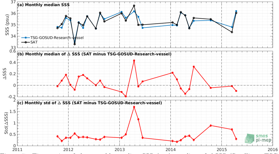
Figure 7: Time series of the monthly median SSS (top), median of \Delta\text{SSS} (Satellite - TSG-GOSUD-Research-vessel) and Std of \Delta\text{SSS} (Satellite - TSG-GOSUD-Research-vessel) over the Equatorial Ocean 10N-10S Pi-MEP region considering all match-ups collected by the Pi-MEP.
