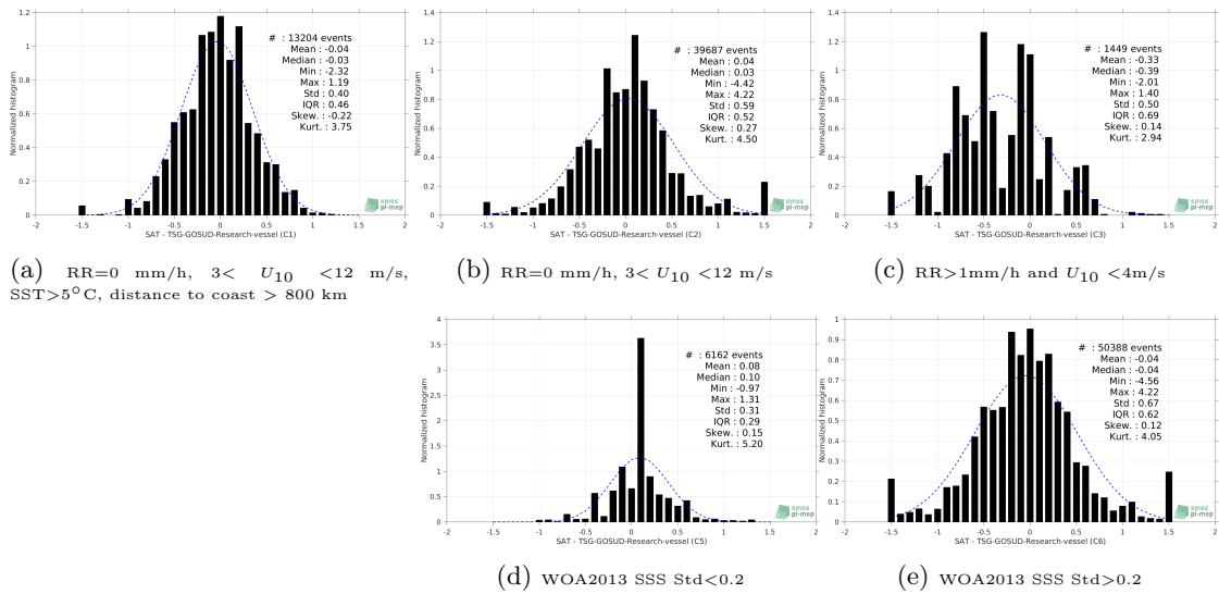
Figure 13: Normalized histogram of \Delta SSS (Aquarius-L2-JPL-V5 - TSG-GOSUD-Research-vessel) for 5 different subdatasets corresponding to: RR=0 mm/h, 3 < U_{10} < 12 m/s, SST >5^\circ C , distance to coast > 800 km (a), RR=0 mm/h, 3 < U_{10} < 12 m/s (b), RR >1 mm/h and U_{10} < 4 m/s (c), WOA2013 SSS Std <0.2 (d), WOA2013 SSS Std >0.2 (e).
