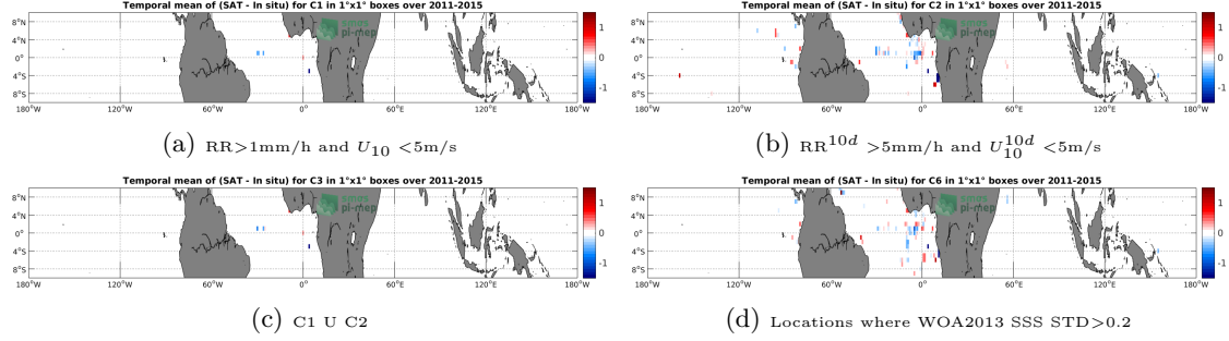
Figure 12: Temporal mean gridded over spatial boxes of size 1^\circ \times 1^\circ of \Delta SSS (Aquarius-L2-JPL-V5 - TSG-GOSUD-Research-vessel) for 4 different subdatasets corresponding to: RR > 1\text{mm/h} and U_{10} < 5\text{m/s} (a), RR^{10d} > 5\text{mm/h} and U_{10}^{10d} < 5\text{m/s} (b), C1 U C2 (c), Locations where WOA2013 SSS STD > 0.2 (d).
