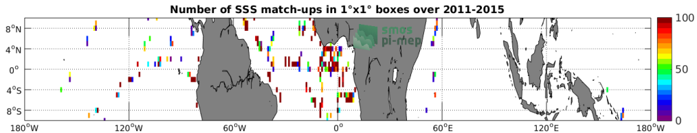
Figure 4: Number of SSS match-ups between TSG-GOSUD-Research-vessel SSS and the Aquarius-L2-JPL-V5 SSS product for the Equatorial Ocean 10N-10S Pi-MEP region over 1^\circ \times 1^\circ boxes and for the full satellite product period.
