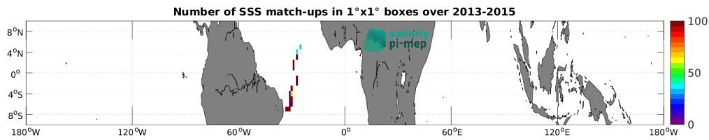
Figure 5: Number of SSS match-ups between TSG (CSIC-UTM) SSS and the Aquarius SSS L2 CAP v5 (JPL) SSS product for the Equatorial Ocean 10N-10S Pi-MEP region over 1^\circ \times 1^\circ boxes and for the full satellite product period.
