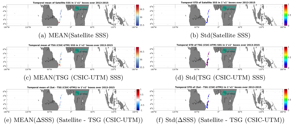
Figure 7: Temporal mean (left) and Std (right) of SSS from Aquarius SSS L2 CAP v5 (JPL) (top), TSG (CSIC-UTM) (middle), and of \Delta SSS (Satellite - TSG (CSIC-UTM)). Only match-up pairs are used to generate these maps.
