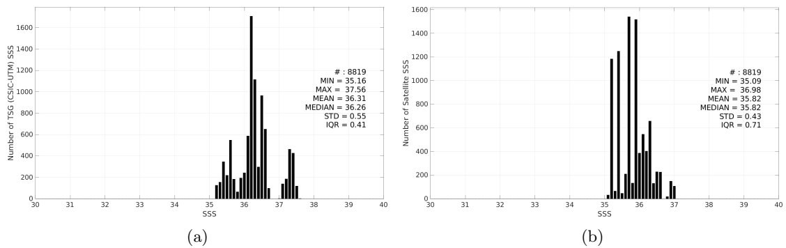
Figure 3: Histograms of SSS from TSG (CSIC-UTM) (a) and Aquarius SSS L2 CAP v5 (JPL) (b) considering all match-up pairs per bins of 0.1 over the Equatorial Ocean 10N-10S Pi-MEP region and for the full satellite product period.
