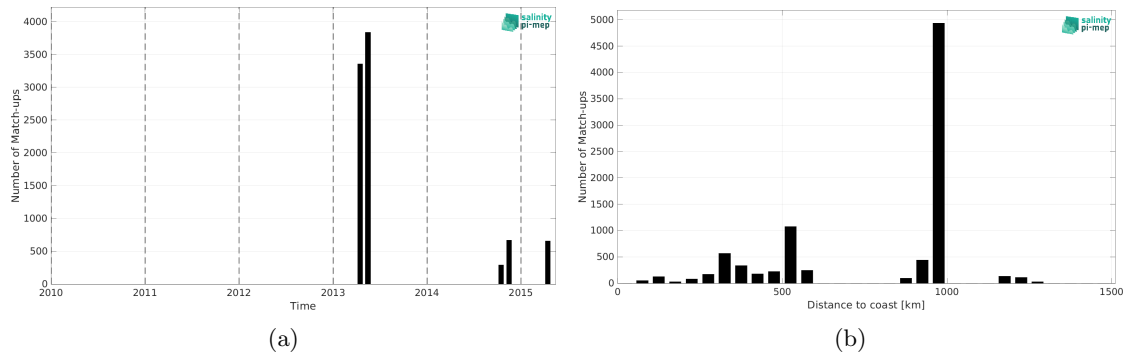
Figure 2: Number of match-ups between TSG (CSIC-UTM) and Aquarius SSS L2 CAP v5 (JPL) SSS as a function of time (a) and as function of the distance to coast (b) over the Equatorial Ocean 10N-10S Pi-MEP region and for the full satellite product period.
