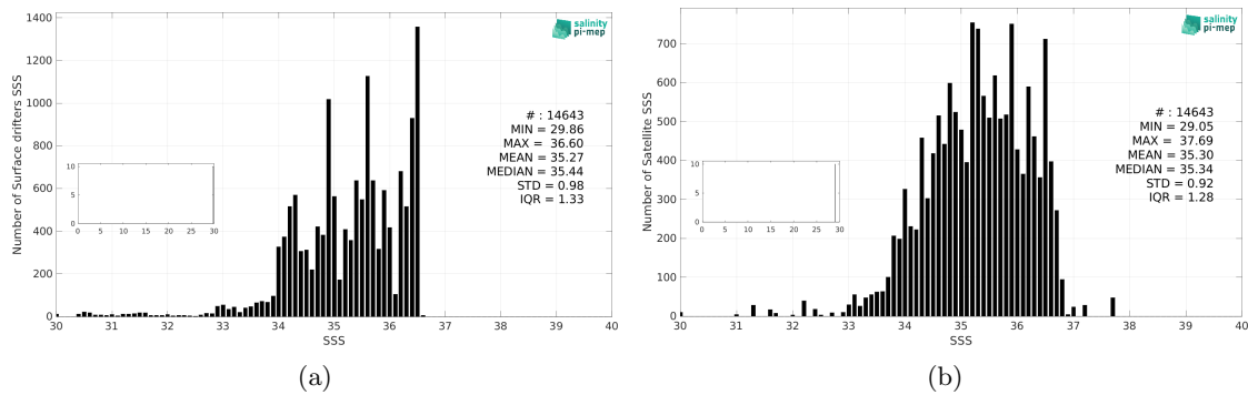
Figure 3: Histograms of SSS from Surface drifters (a) and Aquarius SSS L2 CAP v5 (JPL) (b) considering all match-up pairs per bins of 0.1 over the Equatorial Ocean 10N-10S Pi-MEP region and for the full satellite product period.
