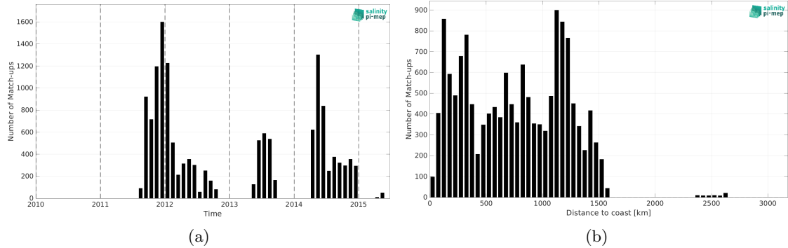
Figure 2: Number of match-ups between Surface drifters and Aquarius SSS L2 CAP v5 (JPL) SSS as a function of time (a) and as function of the distance to coast (b) over the Equatorial Ocean 10N-10S Pi-MEP region and for the full satellite product period.
