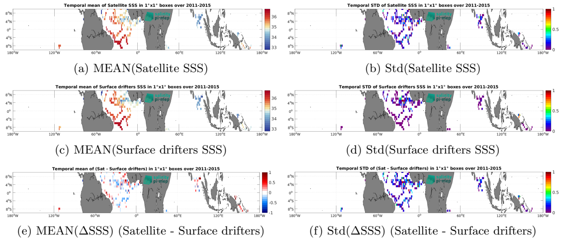
Figure 6: Temporal mean (left) and Std (right) of SSS from Aquarius SSS L2 CAP v5 (JPL) (top), Surface drifters (middle), and of \Delta SSS (Satellite - Surface drifters). Only match-up pairs are used to generate these maps.
