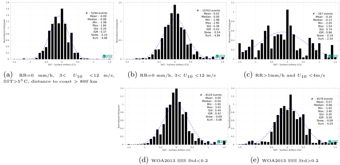
Figure 14: Normalized histogram of \Delta\text{SSS} (Aquarius SSS L2 CAP v5 (JPL) - Surface drifters) for 5 different subdatasets corresponding to: RR=0 mm/h, 3 < U_{10} < 12 m/s, SST >5^\circ\text{C} , distance to coast > 800 km (a), RR=0 mm/h, 3 < U_{10} < 12 m/s (b), RR >1 mm/h and U_{10} < 4 m/s (c), WOA2013 SSS Std <0.2 (d), WOA2013 SSS Std >0.2 (e).
