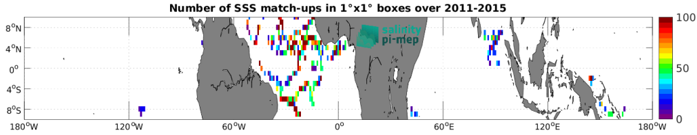
Figure 4: Number of SSS match-ups between Surface drifters SSS and the Aquarius SSS L2 CAP v5 (JPL) SSS product for the Equatorial Ocean 10N-10S Pi-MEP region over 1^\circ \times 1^\circ boxes and for the full satellite product period.
