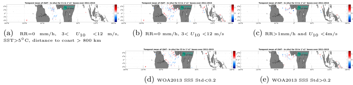
Figure 13: Temporal mean gridded over spatial boxes of size 1^\circ \times 1^\circ of \Delta\text{SSS} (Aquarius SSS L2 CAP v5 (JPL) - Surface drifters) for 5 different subdatasets corresponding to:RR=0 mm/h, 3 < U_{10} < 12 m/s, SST >5^\circ\text{C} , distance to coast > 800 km (a), RR=0 mm/h, 3 < U_{10} < 12 m/s (b), RR >1 mm/h and U_{10} < 4 m/s (c), WOA2013 SSS Std <0.2 (d), WOA2013 SSS Std >0.2 (e).
