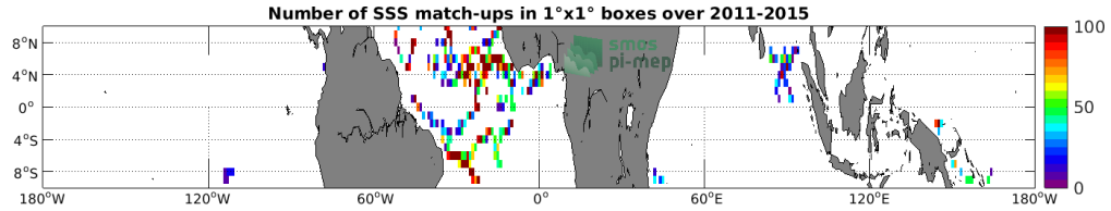
Figure 3: Number of SSS match-ups between Surface drifters SSS and the Aquarius SSS L2 CAP v5 (JPL) SSS product for the Equatorial Ocean 10N-10S Pi-MEP region over 1°x1° boxes and for the full satellite product period.
