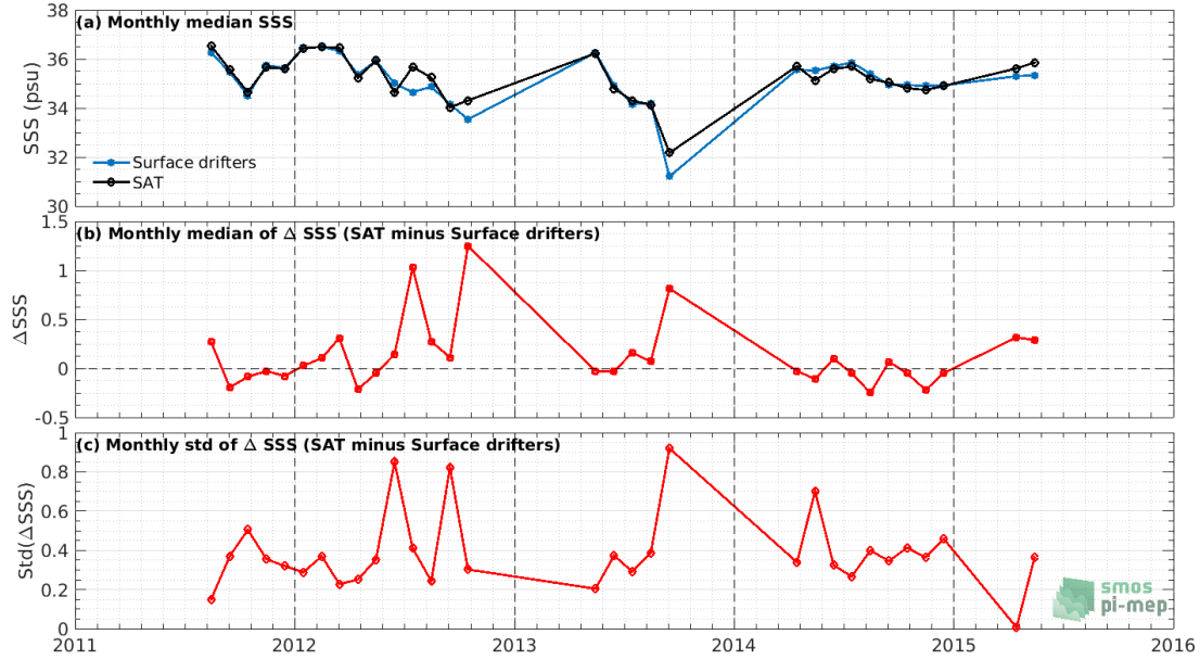
Figure 6: Time series of the monthly median SSS (top), median of \Delta\text{SSS} (Satellite - Surface drifters) and Std of \Delta\text{SSS} (Satellite - Surface drifters) over the Equatorial Ocean 10N-10S Pi-MEP region considering all match-ups collected by the Pi-MEP.
