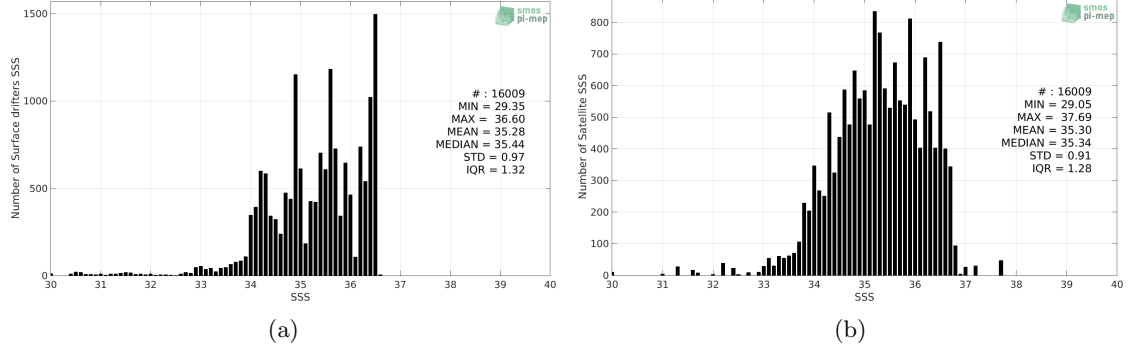
Figure 2: Histograms of SSS from Surface drifters (a) and Aquarius SSS L2 CAP v5 (JPL) (b) considering all match-up pairs per bins of 0.1 over the Equatorial Ocean 10N-10S Pi-MEP region and for the full satellite product period.
