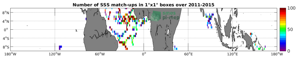
Figure 3: Number of SSS match-ups between Surface drifters SSS and the Aquarius-L2-JPL-V5 SSS product for the Equatorial Ocean 10N-10S Pi-MEP region over 1°x1° boxes and for the full satellite product period.
