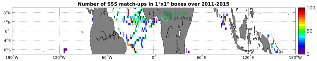
Figure 3: Number of SSS match-ups between Surface drifters SSS and the Aquarius-L2-JPL-V5 SSS product for the Equatorial Ocean 10N-10S Pi-MEP region over 1^\circ \times 1^\circ boxes and for the full satellite product period.
