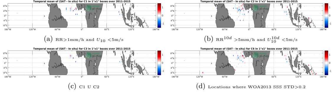
Figure 11: Temporal mean gridded over spatial boxes of size 1^\circ \times 1^\circ of \Delta SSS (Aquarius-L2-JPL-V5 - Surface drifters) for 4 different subdatasets corresponding to: RR > 1\text{mm/h} and U_{10} < 5\text{m/s} (a), RR^{10d} > 5\text{mm/h} and U_{10}^{10d} < 5\text{m/s} (b), C1 U C2 (c), Locations where WOA2013 SSS STD > 0.2 (d).
