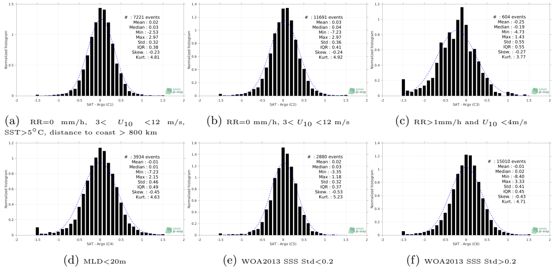
Figure 13: Normalized histogram of \Delta SSS (Aquarius SSS L2 CAP v5 (JPL) - Argo) for 6 different subdatasets corresponding to: RR=0 mm/h, 3 < U_{10} < 12 m/s, SST >5^\circ\text{C} , distance to coast > 800 km (a), RR=0 mm/h, 3 < U_{10} < 12 m/s (b), RR >1 mm/h and U_{10} < 4 m/s (c), MLD <20 m (d), WOA2013 SSS Std <0.2 (e), WOA2013 SSS Std >0.2 (f).
