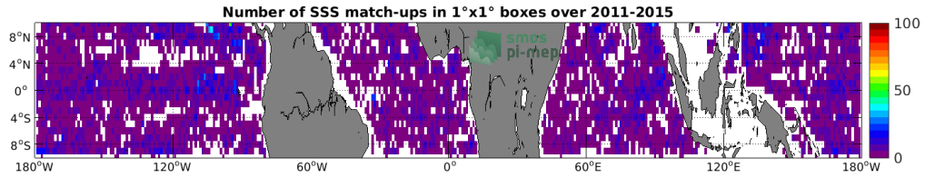
Figure 4: Number of SSS match-ups between Argo SSS and the Aquarius SSS L2 CAP v5 (JPL) SSS product for the Equatorial Ocean 10N-10S Pi-MEP region over 1°x1° boxes and for the full satellite product period.
