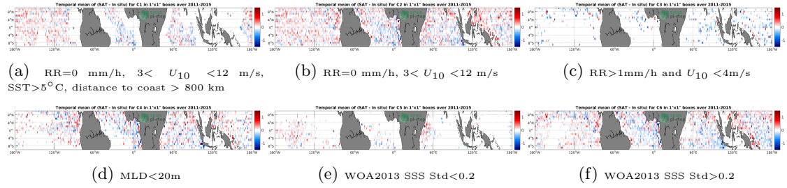
Figure 12: Temporal mean gridded over spatial boxes of size 1^\circ \times 1^\circ of \Delta SSS (Aquarius-L2-JPL-V5 - Argo) for 6 different subdatasets corresponding to:RR=0 mm/h, 3 < U_{10} < 12 m/s, SST >5^\circ\text{C} , distance to coast > 800 km (a), RR=0 mm/h, 3 < U_{10} < 12 m/s (b), RR >1 mm/h and U_{10} < 4 m/s (c),MLD <20 m (d),WOA2013 SSS Std <0.2 (e),WOA2013 SSS Std >0.2 (f).
