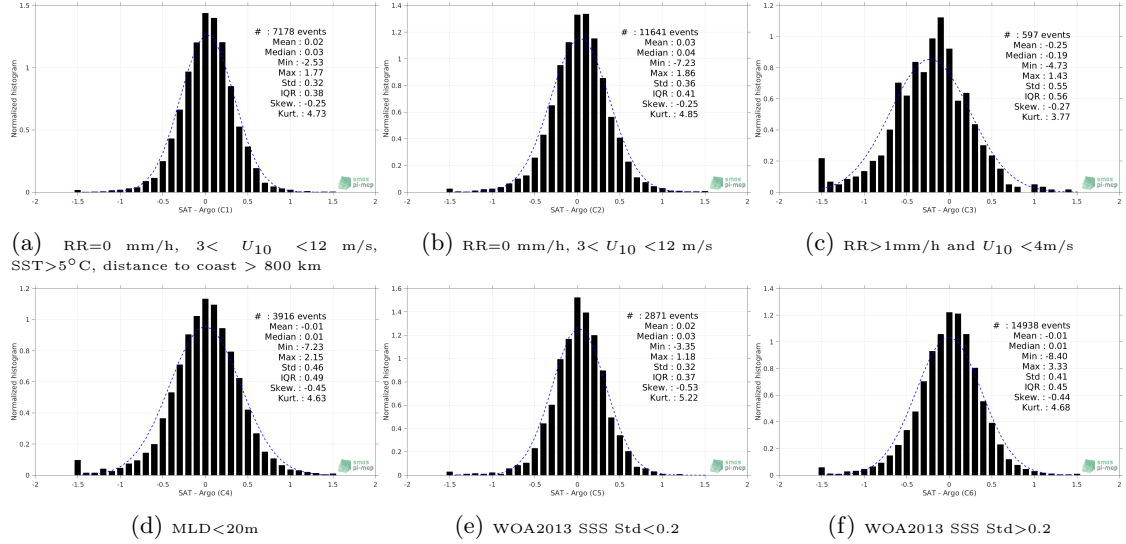
Figure 13: Normalized histogram of \Delta SSS (Aquarius-L2-JPL-V5 - Argo) for 6 different subdatasets corresponding to: RR=0 mm/h, 3 < U_{10} < 12 m/s, SST >5^\circ\text{C} , distance to coast > 800 km (a), RR=0 mm/h, 3 < U_{10} < 12 m/s (b), RR >1 mm/h and U_{10} < 4 m/s (c), MLD <20 m (d), WOA2013 SSS Std <0.2 (e), WOA2013 SSS Std >0.2 (f).
