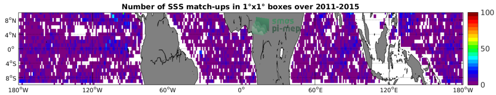
Figure 4: Number of SSS match-ups between Argo SSS and the Aquarius-L2-JPL-V5 SSS product for the Equatorial Ocean 10N-10S Pi-MEP region over 1^\circ \times 1^\circ boxes and for the full satellite product period.
