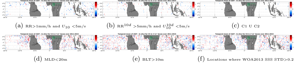
Figure 12: Temporal mean gridded over spatial boxes of size 1^\circ \times 1^\circ of \Delta\text{SSS} (Aquarius-L2-JPL-V5 - Argo) for 6 different subdatasets corresponding to: \text{RR} > 1\text{mm/h} and U_{10} < 5\text{m/s} (a), \text{RR}^{10d} > 5\text{mm/h} and U_{10}^{10d} < 5\text{m/s} (b), C1 U C2 (c), \text{MLD} < 20\text{m} (d), \text{BLT} > 10\text{m} (e), Locations where WOA2013 SSS STD > 0.2 (f).
