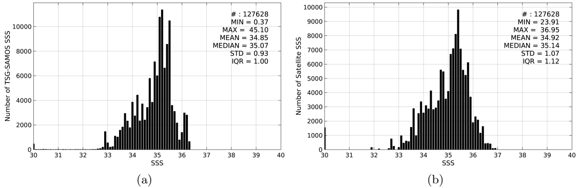
Figure 2: Histograms of SSS from TSG-SAMOS (a) and AQUARIUS-L2-JPL-V4 (b) considering all match-up pairs per bins of 0.1 over the Equatorial Ocean 10N-10S Pi-MEP region and for the full satellite product period.
