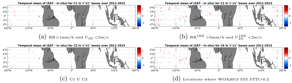
Figure 12: Temporal mean gridded over spatial boxes of size 1^\circ \times 1^\circ of \Delta SSS (AQUARIUS-L2-JPL-V4 - TSG-SAMOS) for 4 different subdatasets corresponding to: RR > 1\text{mm/h} and U_{10} < 5\text{m/s} (a), RR^{10d} > 5\text{mm/h} and U_{10}^{10d} < 5\text{m/s} (b), C1 U C2 (c), Locations where WOA2013 SSS STD > 0.2 (d).
