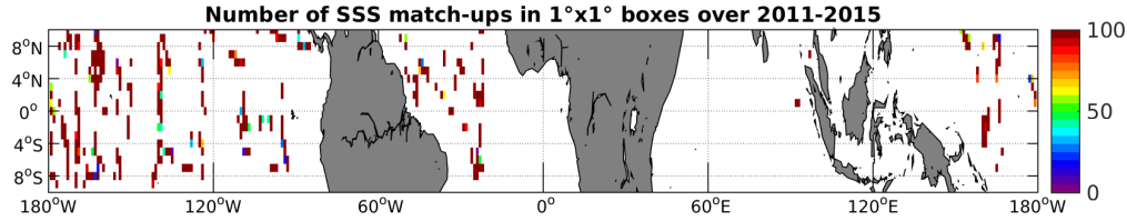
Figure 4: Number of SSS match-ups between TSG-SAMOS SSS and the AQUARIUS-L2-JPL-V4 SSS product for the Equatorial Ocean 10N-10S Pi-MEP region over 1^\circ \times 1^\circ boxes and for the full satellite product period.
