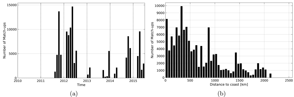
Figure 1: Number of match-ups between TSG-SAMOS and AQUARIUS-L2-JPL-V4 SSS as a function of time (a) and as function of the distance to coast (b) over the Equatorial Ocean 10N-10S Pi-MEP region and for the full satellite product period.
