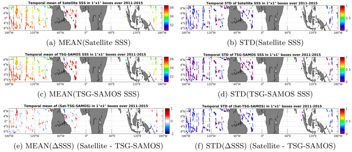
Figure 6: Temporal mean (left) and STD (right) of SSS from AQUARIUS-L2-JPL-V4 (top), TSG-SAMOS (middle), and of \Delta SSS (Satellite - TSG-SAMOS). Only match-up pairs are used to generate these maps.
