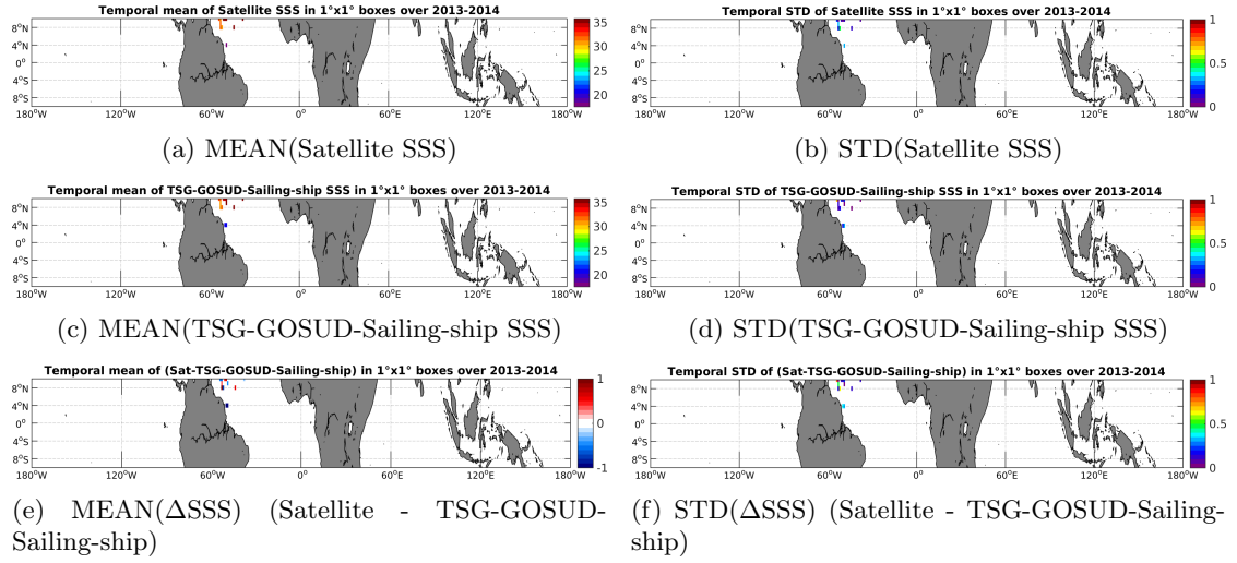
Figure 6: Temporal mean (left) and STD (right) of SSS from AQUARIUS-L2-JPL-V4 (top), TSG-GOSUD-Sailing-ship (middle), and of \Delta SSS (Satellite - TSG-GOSUD-Sailing-ship). Only match-up pairs are used to generate these maps.
