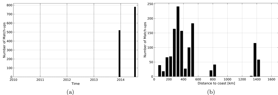
Figure 1: Number of match-ups between TSG-GOSUD-Sailing-ship and AQUARIUS-L2-JPL-V4 SSS as a function of time (a) and as function of the distance to coast (b) over the Equatorial Ocean 10N-10S Pi-MEP region and for the full satellite product period.
