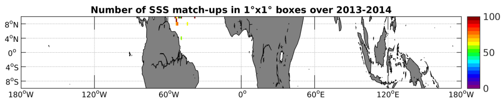
Figure 4: Number of SSS match-ups between TSG-GOSUD-Sailing-ship SSS and the AQUARIUS-L2-JPL-V4 SSS product for the Equatorial Ocean 10N-10S Pi-MEP region over 1^\circ \times 1^\circ boxes and for the full satellite product period.
