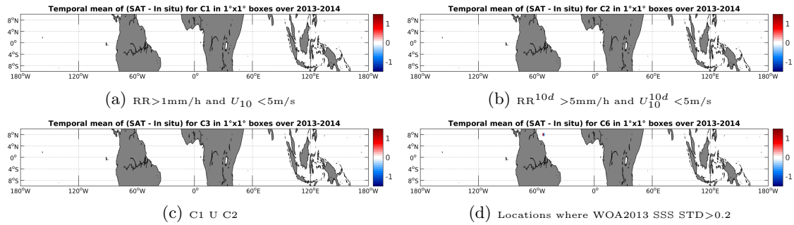
Figure 12: Temporal mean gridded over spatial boxes of size 1^\circ \times 1^\circ of \Delta SSS (AQUARIUS-L2-JPL-V4 - TSG-GOSUD-Sailing-ship) for 4 different subdatasets corresponding to: RR > 1\text{mm/h} and U_{10} < 5\text{m/s} (a), RR^{10d} > 5\text{mm/h} and U_{10}^{10d} < 5\text{m/s} (b), C1 U C2 (c), Locations where WOA2013 SSS STD > 0.2 (d).
