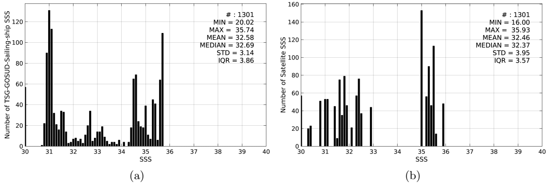
Figure 2: Histograms of SSS from TSG-GOSUD-Sailing-ship (a) and AQUARIUS-L2-JPL-V4 (b) considering all match-up pairs per bins of 0.1 over the Equatorial Ocean 10N-10S Pi-MEP region and for the full satellite product period.
