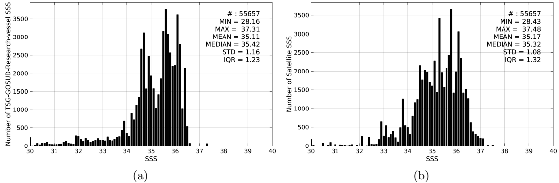
Figure 2: Histograms of SSS from TSG-GOSUD-Research-vessel (a) and AQUARIUS-L2-JPL-V4 (b) considering all match-up pairs per bins of 0.1 over the Equatorial Ocean 10N-10S Pi-MEP region and for the full satellite product period.
