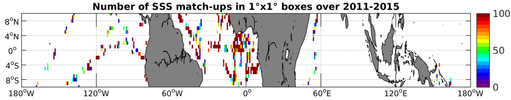
Figure 4: Number of SSS match-ups between TSG-GOSUD-Research-vessel SSS and the AQUARIUS-L2-JPL-V4 SSS product for the Equatorial Ocean 10N-10S Pi-MEP region over 1^\circ \times 1^\circ boxes and for the full satellite product period.
