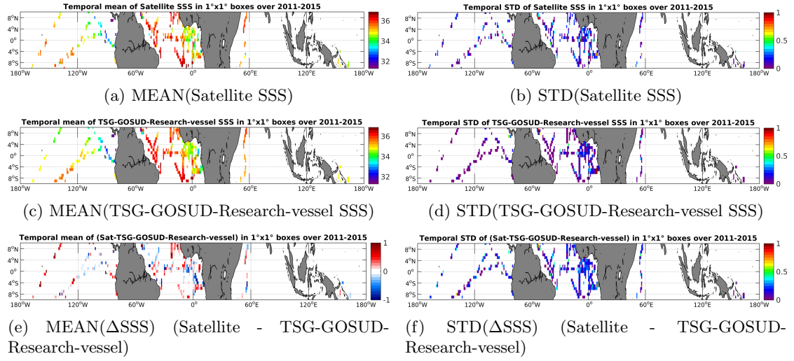
Figure 6: Temporal mean (left) and STD (right) of SSS from AQUARIUS-L2-JPL-V4 (top), TSG-GOSUD-Research-vessel (middle), and of \Delta SSS (Satellite - TSG-GOSUD-Research-vessel). Only match-up pairs are used to generate these maps.
