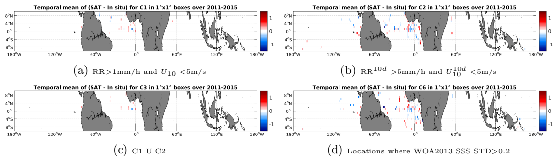
Figure 12: Temporal mean gridded over spatial boxes of size 1^\circ \times 1^\circ of \Delta SSS (AQUARIUS-L2-JPL-V4 - TSG-GOSUD-Research-vessel) for 4 different subdatasets corresponding to: RR > 1 mm/h and U_{10} < 5 m/s (a), RR^{10d} > 5 mm/h and U_{10}^{10d} < 5 m/s (b), C1 U C2 (c), Locations where WOA2013 SSS STD > 0.2 (d).
