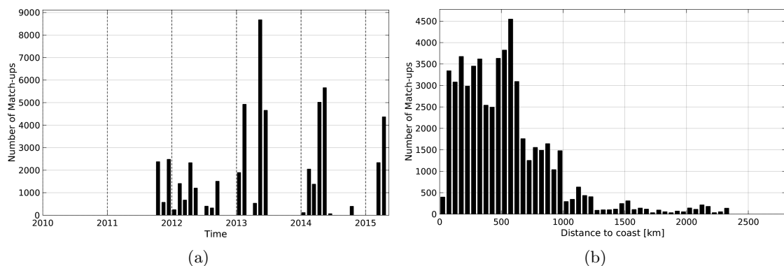
Figure 1: Number of match-ups between TSG-GOSUD-Research-vessel and AQUARIUS-L2-JPL-V4 SSS as a function of time (a) and as function of the distance to coast (b) over the Equatorial Ocean 10N-10S Pi-MEP region and for the full satellite product period.
