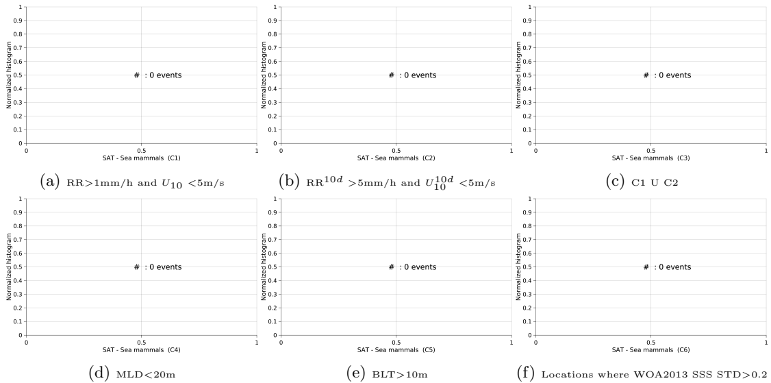
Figure 13: Normalized histogram of ΔSSS (AQUARIUS-L2-JPL-V4 - Sea mammals) for 6 different subdatasets corresponding to: RR>1mm/h and U_{10} < 5\text{m/s} (a), RR^{10d} > 5\text{mm/h} and U_{10}^{10d} < 5\text{m/s} (b), C1 U C2 (c),MLD<20m (d),BLT>10m (e),Locations where WOA2013 SSS STD>0.2 (f).
