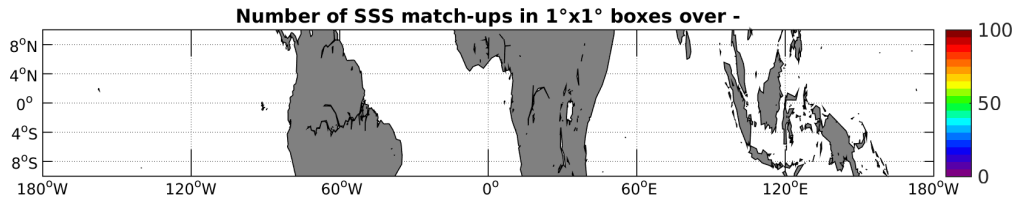
Figure 4: Number of SSS match-ups between Sea mammals SSS and the AQUARIUS-L2-JPL-V4 SSS product for the Equatorial Ocean 10N-10S Pi-MEP region over 1^\circ \times 1^\circ boxes and for the full satellite product period.
