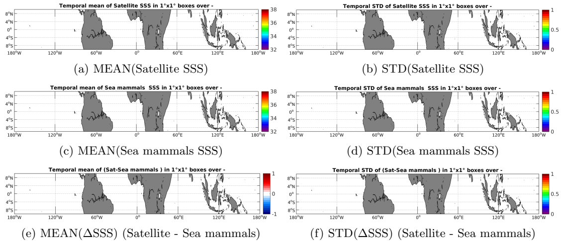
Figure 6: Temporal mean (left) and STD (right) of SSS from AQUARIUS-L2-JPL-V4 (top), Sea mammals (middle), and of \Delta SSS (Satellite - Sea mammals). Only match-up pairs are used to generate these maps.
