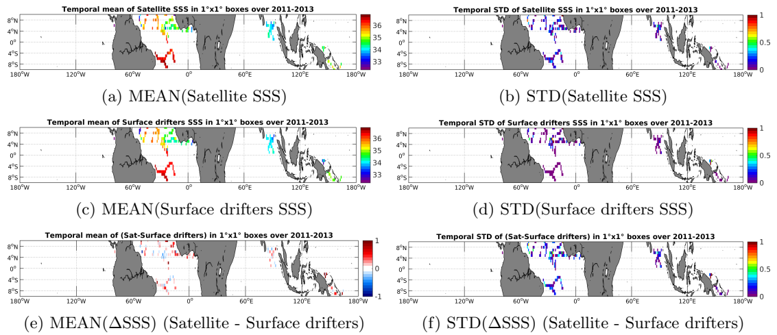
Figure 5: Temporal mean (left) and STD (right) of SSS from AQUARIUS-L2-JPL-V4 (top), Surface drifters (middle), and of \Delta SSS (Satellite - Surface drifters). Only match-up pairs are used to generate these maps.
