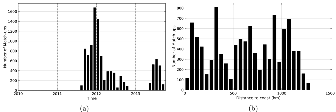
Figure 1: Number of match-ups between Surface drifters and AQUARIUS-L2-JPL-V4 SSS as a function of time (a) and as function of the distance to coast (b) over the Equatorial Ocean 10N-10S Pi-MEP region and for the full satellite product period.
