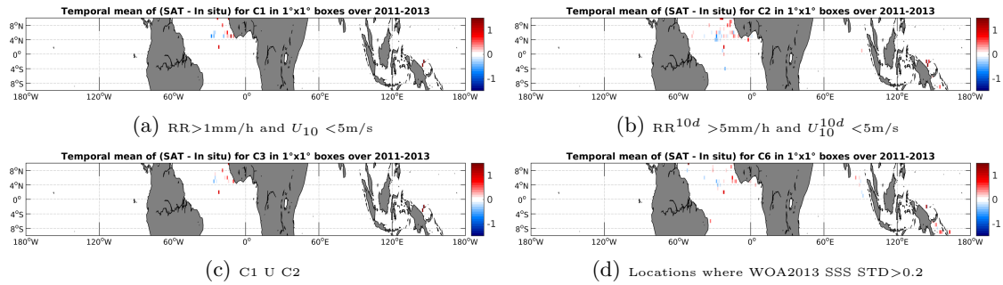
Figure 11: Temporal mean gridded over spatial boxes of size 1^\circ \times 1^\circ of \Delta SSS (AQUARIUS-L2-JPL-V4 - Surface drifters) for 4 different subdatasets corresponding to: RR > 1\text{mm/h} and U_{10} < 5\text{m/s} (a), RR^{10d} > 5\text{mm/h} and U_{10}^{10d} < 5\text{m/s} (b), C1 U C2 (c), Locations where WOA2013 SSS STD > 0.2 (d).
