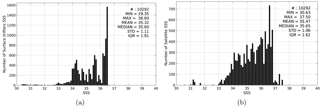
Figure 2: Histograms of SSS from Surface drifters (a) and AQUARIUS-L2-JPL-V4 (b) considering all match-up pairs per bins of 0.1 over the Equatorial Ocean 10N-10S Pi-MEP region and for the full satellite product period.
