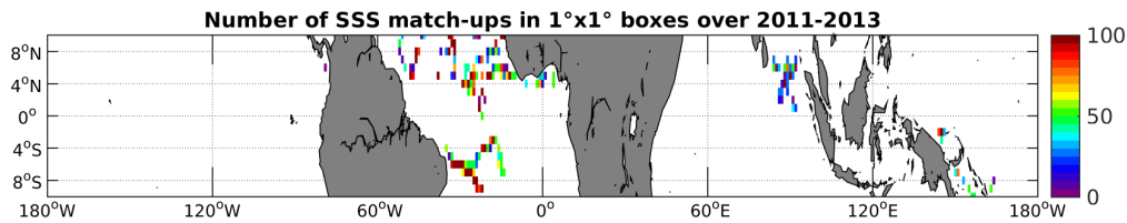
Figure 3: Number of SSS match-ups between Surface drifters SSS and the AQUARIUS-L2-JPL-V4 SSS product for the Equatorial Ocean 10N-10S Pi-MEP region over 1^\circ \times 1^\circ boxes and for the full satellite product period.
