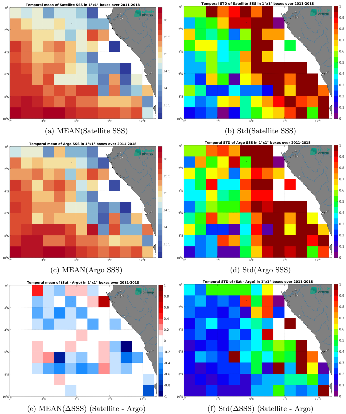
Figure 6: Temporal mean (left) and Std (right) of SSS from SMOS and SMAP SSS L4 OI v1 - 7 Days (LOPS) (top), Argo (middle), and of \Delta SSS (Satellite - Argo). Only match-up pairs are used to generate these maps.
