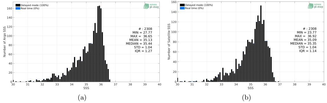
Figure 2: Histograms of SSS from Argos (a) and SMOS and SMAP SSS L4 OI v1 - 7 Days (LOPS) (b) considering all match-up pairs per bins of 0.1 over the Congo river plume Pi-MEP region and for the full satellite product period.
