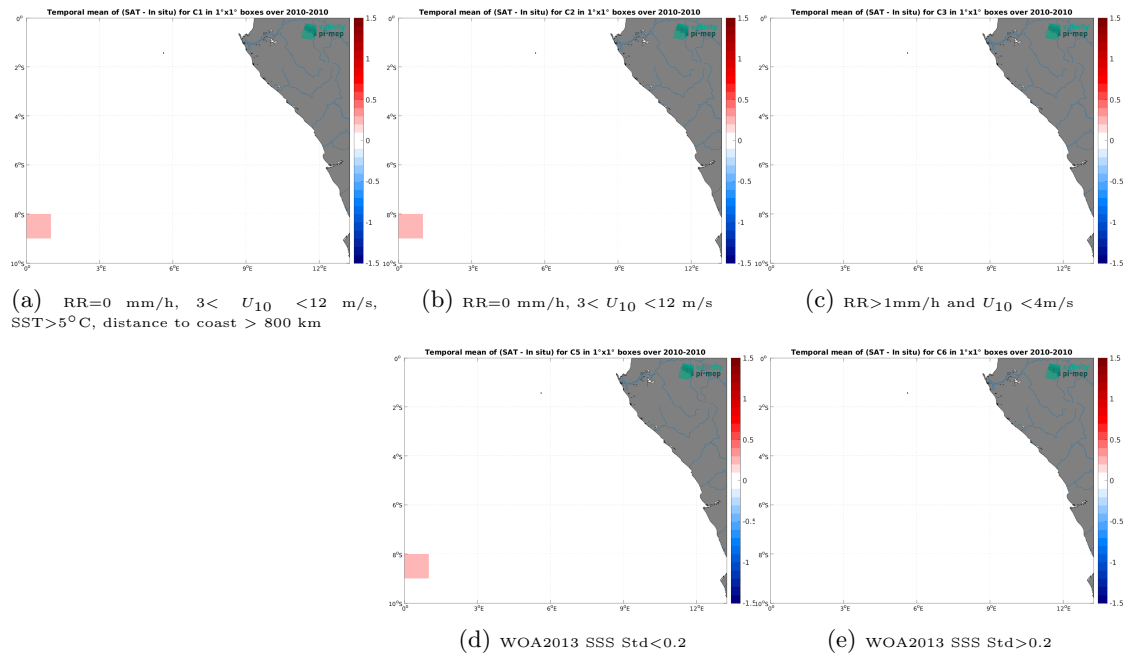
Figure 12: Temporal mean gridded over spatial boxes of size 1^\circ \times 1^\circ of \Delta SSS (SMOS SSS L4 v1 - Weekly (CMEMS-CNR) - TSG (SAMOS)) for 5 different subdatasets corresponding to: RR=0 mm/h, 3 < U_{10} < 12 m/s, SST > 5^\circ C , distance to coast > 800 km (a), RR=0 mm/h, 3 < U_{10} < 12 m/s (b), RR > 1 mm/h and U_{10} < 4 m/s (c), WOA2013 SSS Std < 0.2 (d), WOA2013 SSS Std > 0.2 (e).
