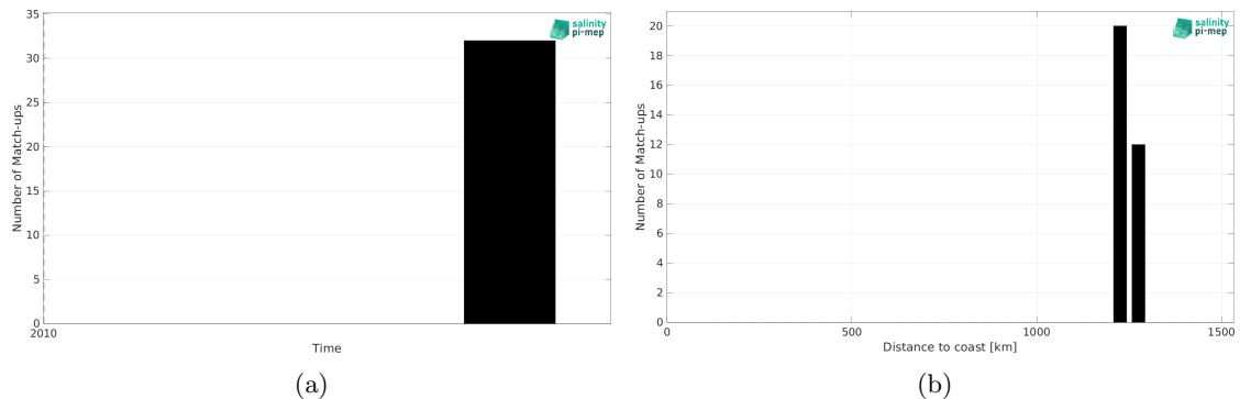
Figure 1: Number of match-ups between TSG (SAMOS) and SMOS SSS L4 v1 - Weekly (CMEMS-CNR) SSS as a function of time (a) and as function of the distance to coast (b) over the Congo river plume Pi-MEP region and for the full satellite product period.
