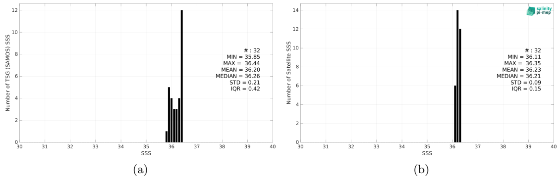
Figure 2: Histograms of SSS from TSG (SAMOS) (a) and SMOS SSS L4 v1 - Weekly (CMEMS-CNR) (b) considering all match-up pairs per bins of 0.1 over the Congo river plume Pi-MEP region and for the full satellite product period.
