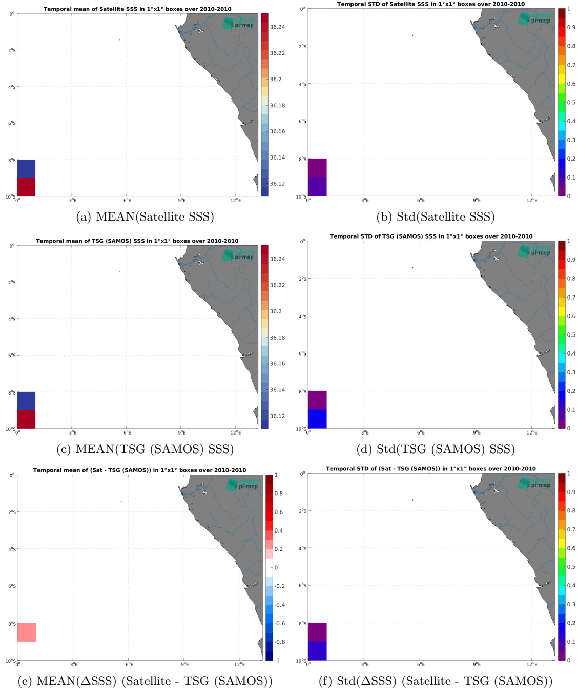
Figure 6: Temporal mean (left) and Std (right) of SSS from SMOS SSS L4 v1 - Weekly (CMEMS-CNR) (top), TSG (SAMOS) (middle), and of \Delta SSS (Satellite - TSG (SAMOS)). Only match-up pairs are used to generate these maps.
