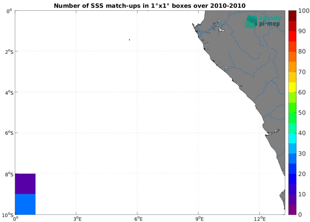
Figure 4: Number of SSS match-ups between TSG (SAMOS) SSS and the SMOS SSS L4 v1 - Weekly (CMEMS-CNR) SSS product for the Congo river plume Pi-MEP region over 1°x1° boxes and for the full satellite product period.
