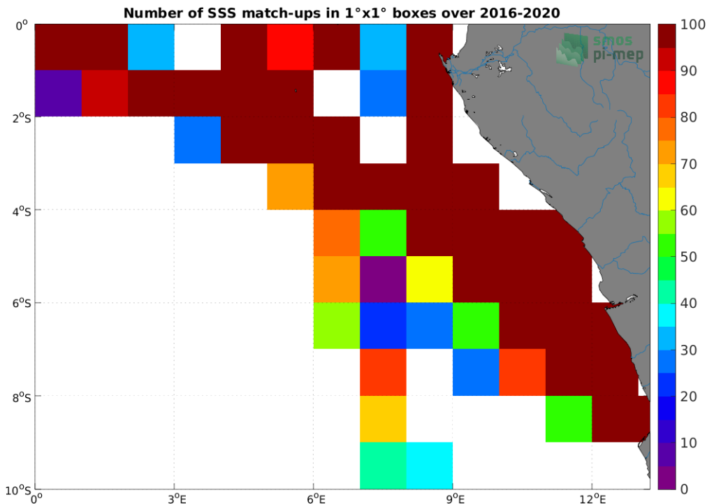
Figure 4: Number of SSS match-ups between TSG (LEGOS-DM) SSS and the SMOS SSS L4 v1 - Weekly (CMEMS-CNR) SSS product for the Congo river plume Pi-MEP region over 1^\circ \times 1^\circ boxes and for the full satellite product period.
